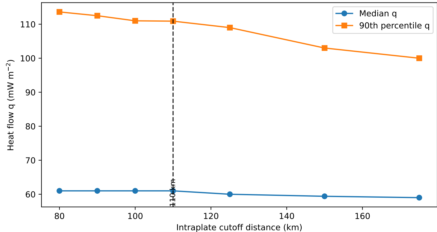
Sensitivity of thermal statistics to distance cutoff
