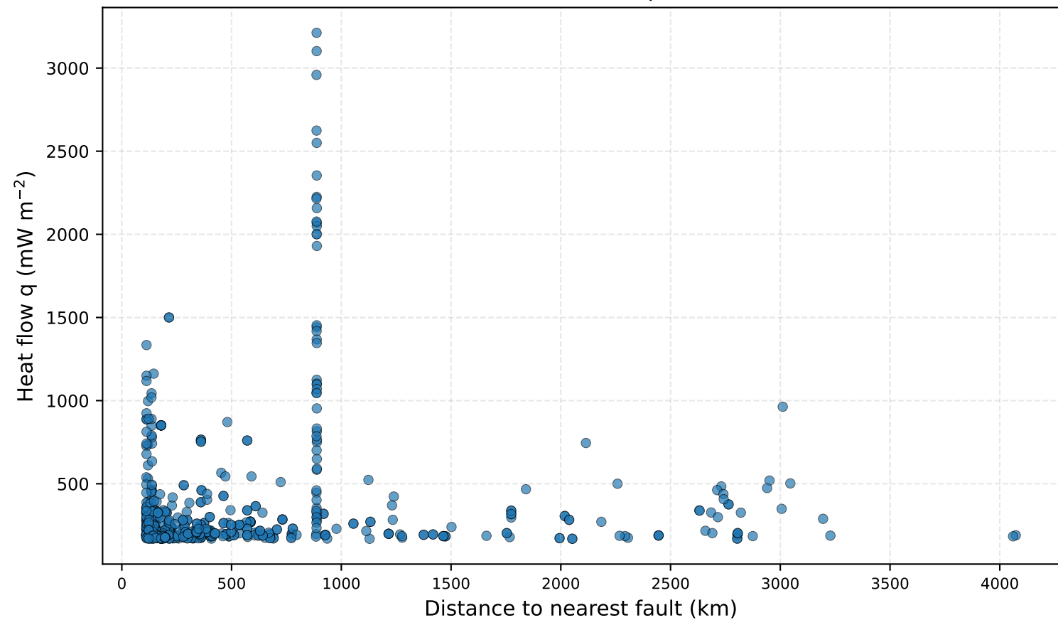
Distance vs heat flow for final intraplate outliers (n = 603)
