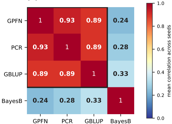
(A) How alike do the methods behave?
