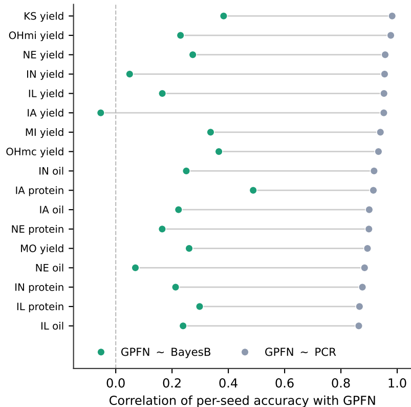
(B) GPFN moves with its projection, not with BayesB
