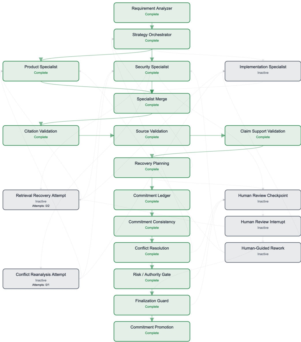
Figure 2. Actual offline RFP-002 execution-map capture: Product and Security completed as independent peers, Implementation inactive; observed arrows lead through merge and guarded finalization. Unused recovery and HITL routes stay gray. [9]
