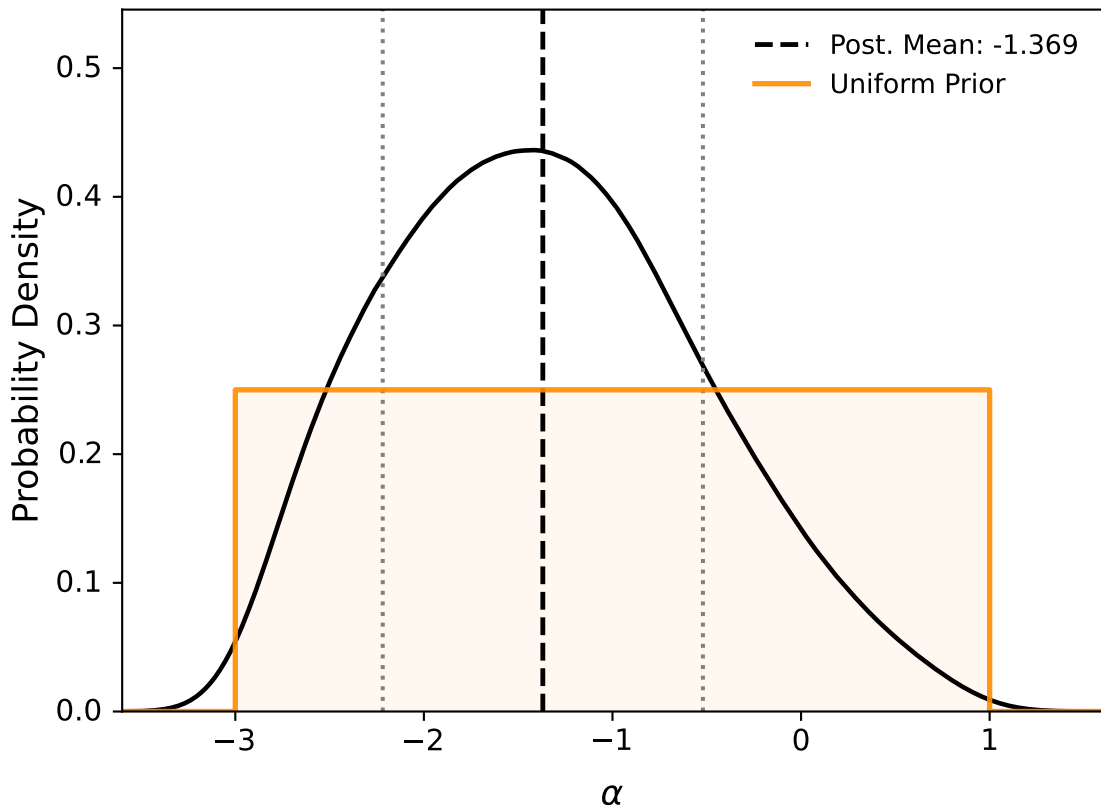
Figure: Constraint on \alpha with best-fit value -1.369 \pm 0.849
