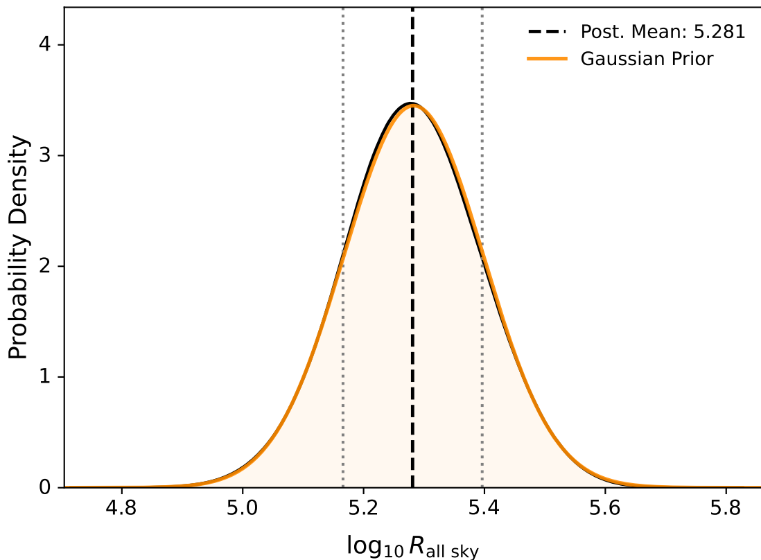
Figure: Constraint on \log_{10} R_{\text{all sky}} with best-fit value 5.281 \pm 0.115
