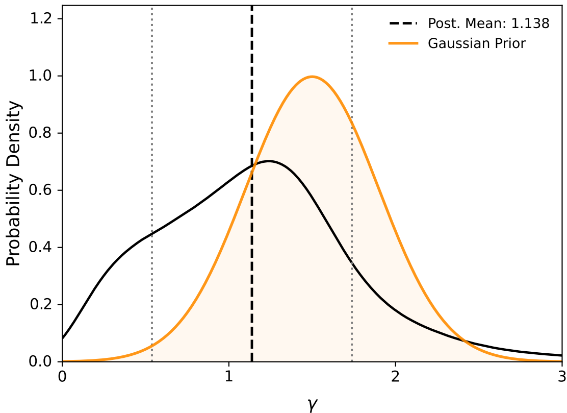
Figure: Constraint on \gamma with best-fit value 1.138 \pm 0.600
