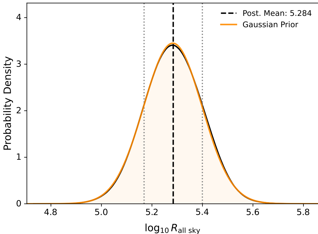
Figure: Constraint on \log_{10} R_{\text{all sky}} with best-fit value 5.284 \pm 0.115
