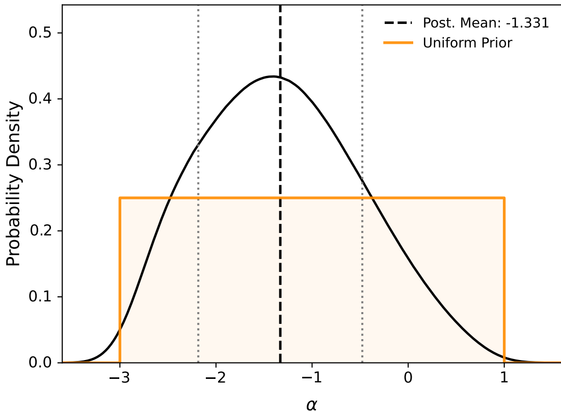
Figure: Constraint on \alpha with best-fit value -1.331 \pm 0.853
