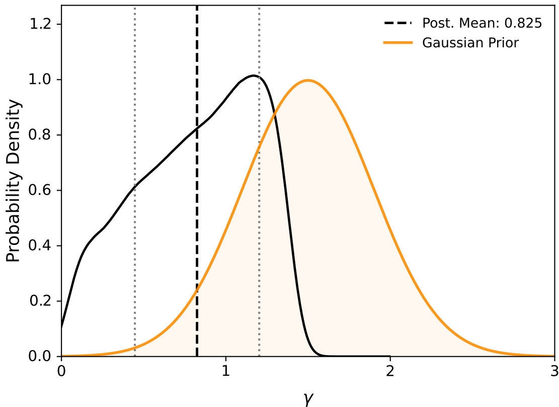
Figure: Constraint on \gamma with best-fit value 0.825 \pm 0.378
