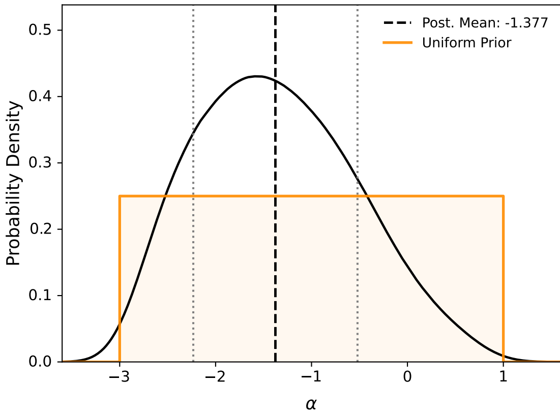
Figure: Constraint on \alpha with best-fit value -1.377 \pm 0.856
