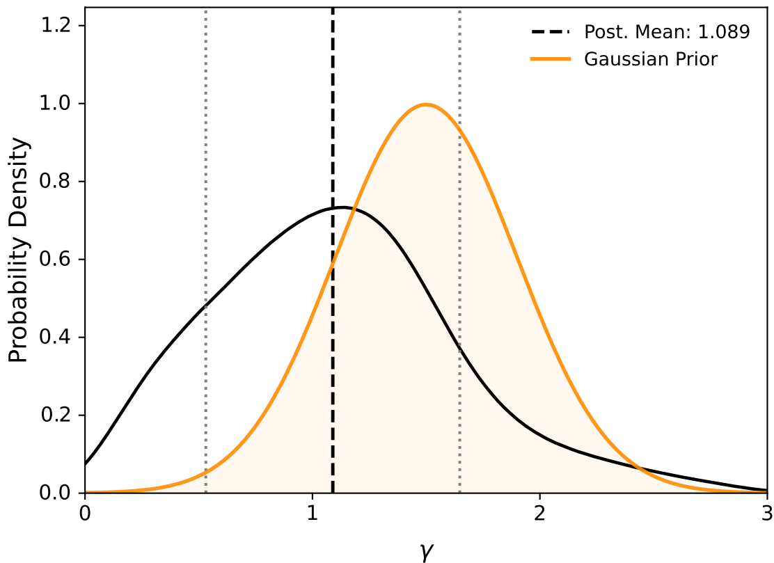
Figure: Constraint on \gamma with best-fit value 1.089 \pm 0.558
