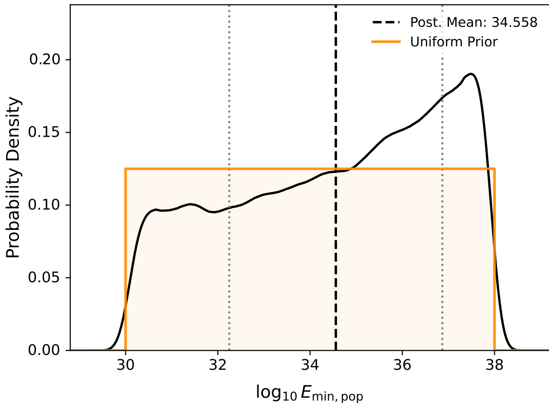
Figure: Constraint on \log_{10} E_{\text{min, pop}} with best-fit value 34.558 \pm 2.310
