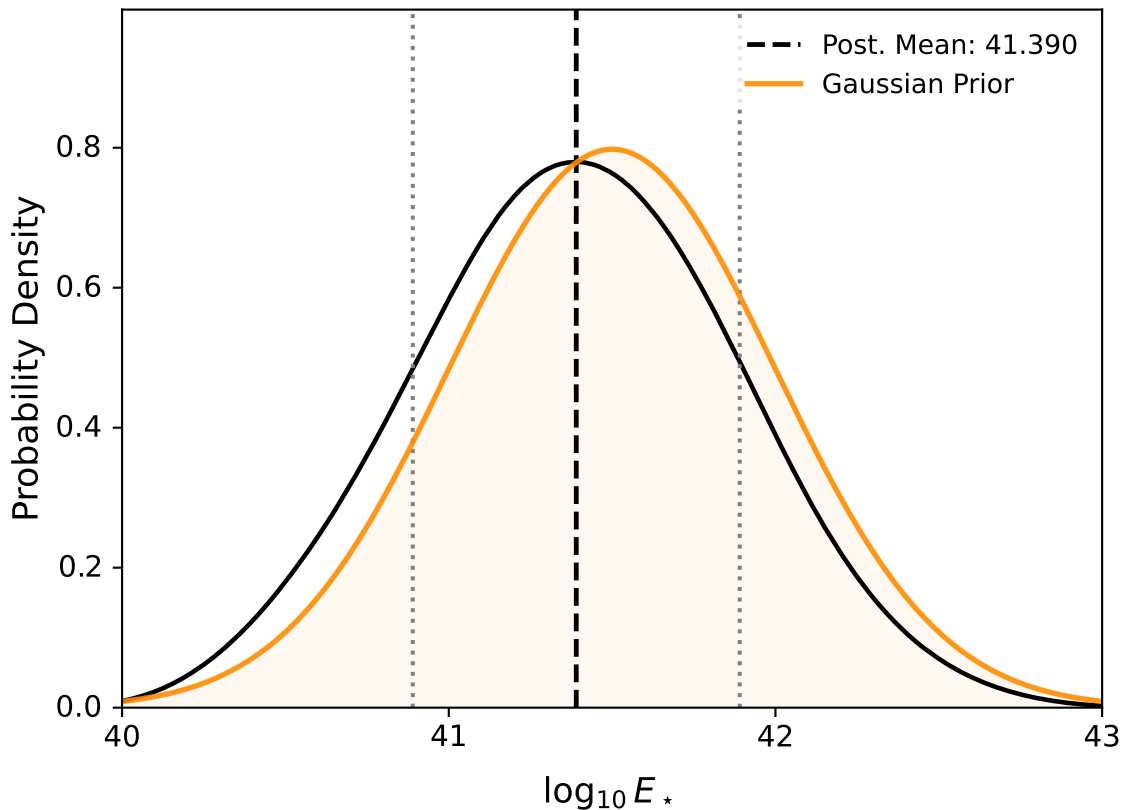
Figure: Constraint on \log_{10} E_* with best-fit value 41.390 \pm 0.500
