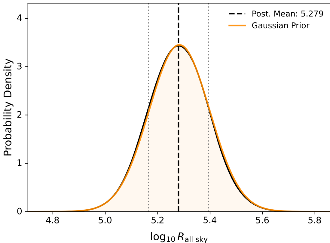
Figure: Constraint on \log_{10} R_{\text{all sky}} with best-fit value 5.279 \pm 0.115
