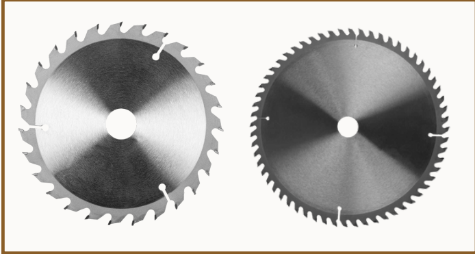
HSS & TCT Saws
