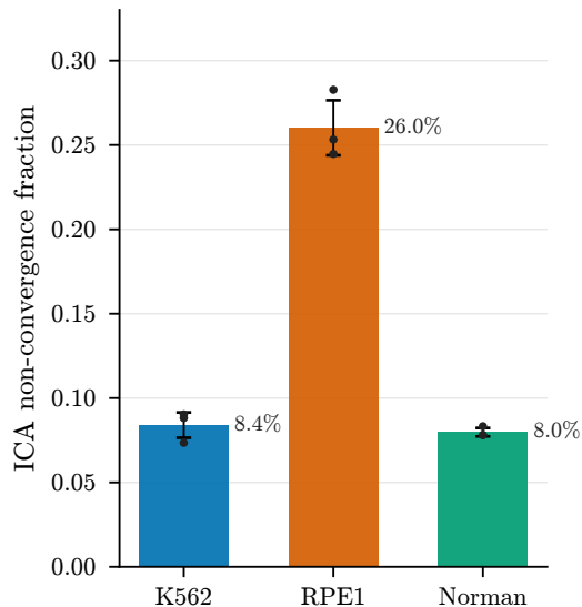
(b) ICA non-convergence is highest on RPE1
