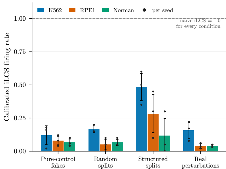
(a) Size matching reduces iLCS firing on pure-control resamples
