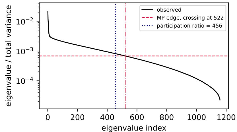
k562 n=2000, p=1158 rank 1158/1158
