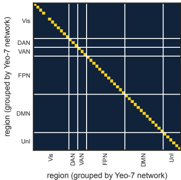
A ABIDE-I site: 49 diagonal, 0 off-diagonal
