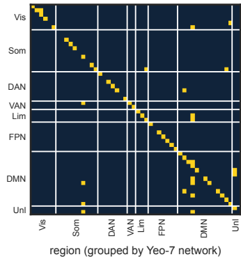
B ADHD-200 site: 39 diagonal, 20 off-diagonal
