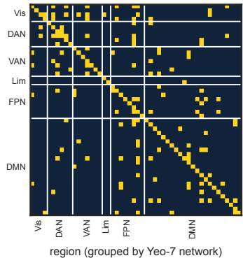
C AOMIC condition: 50 diagonal, 129 off-diagonal
