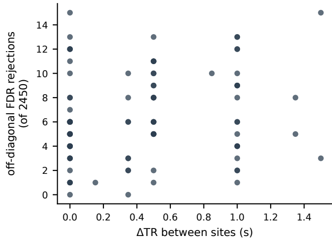
B Off-diagonal (control) Spearman \rho=+0.17 , p=0.11
