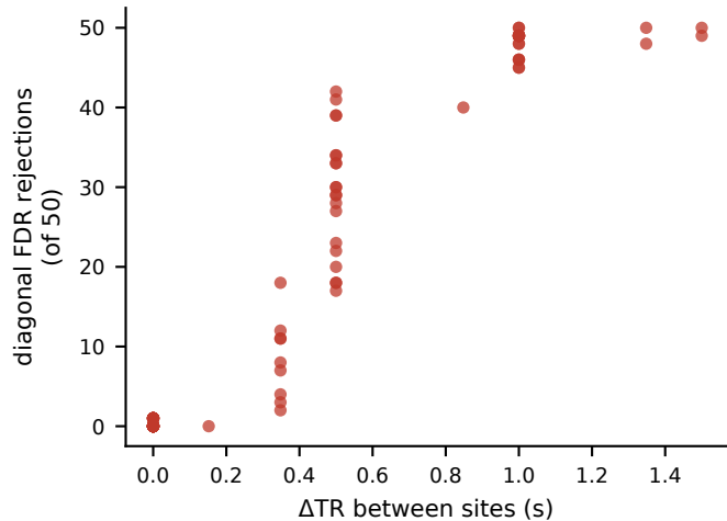
A Diagonal (self-loops) Spearman \rho=+0.96 , p=5.3\text{e-}49
