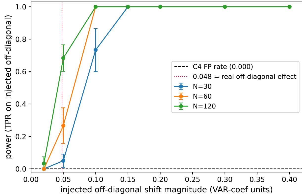
Off-diagonal detection power (C2)
