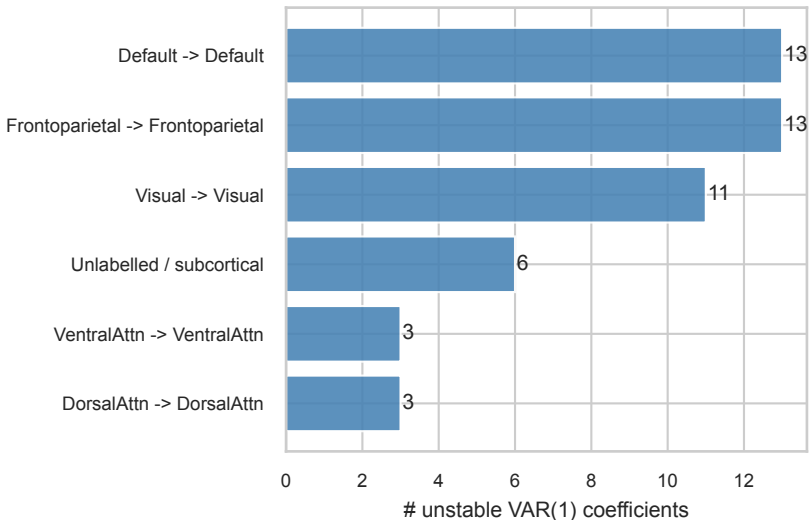
ABIDE-I unstable coefficients by Yeo 7-network (source j -> target i)
