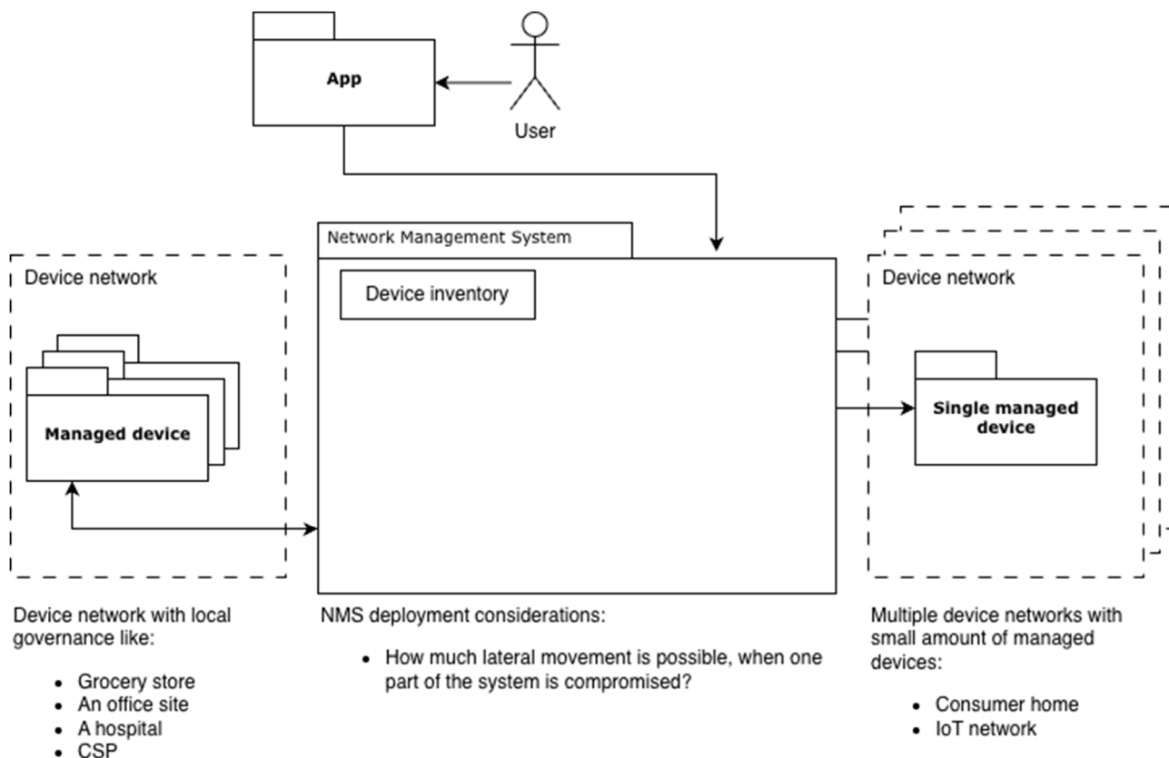
Figure 4.2.1-1: Network distribution design
