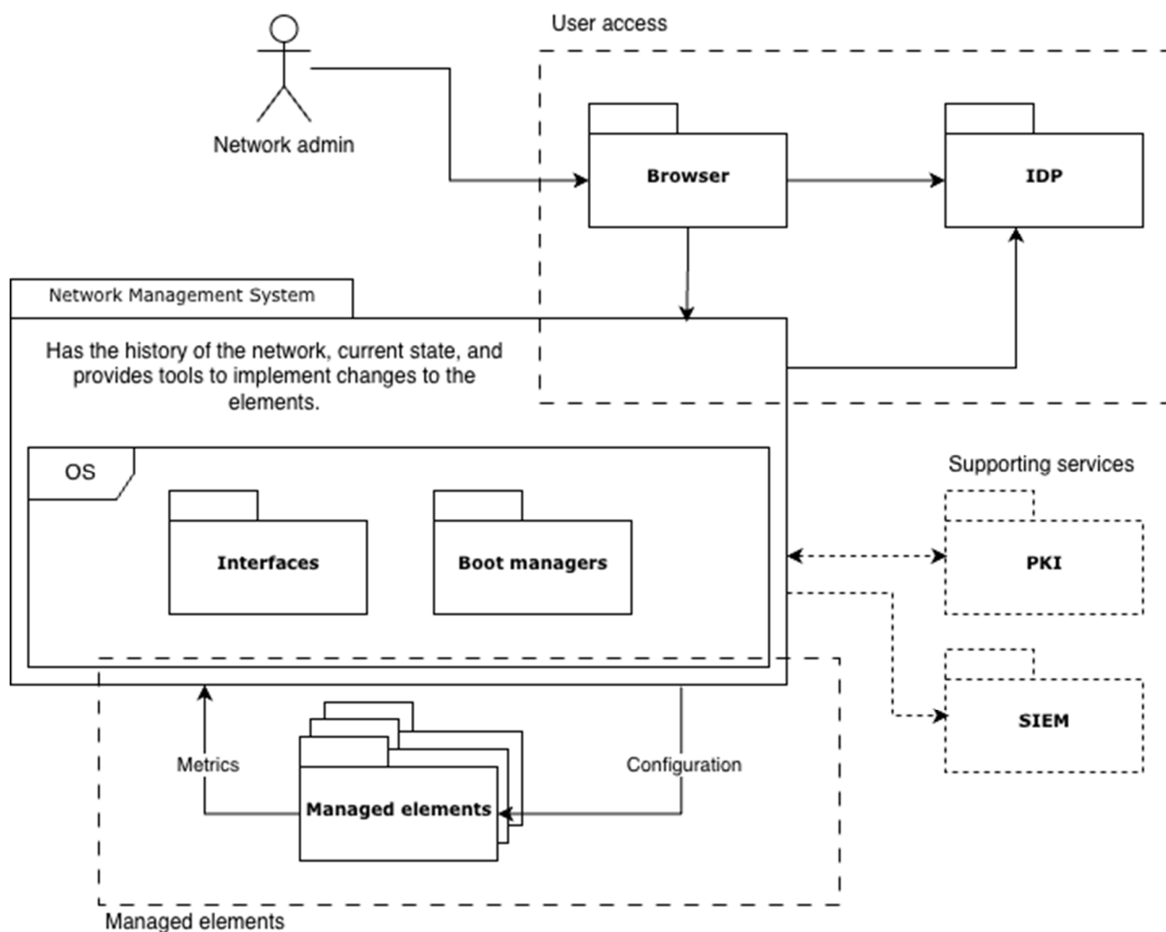
Figure 4.2.0-1: Product overview and architecture
