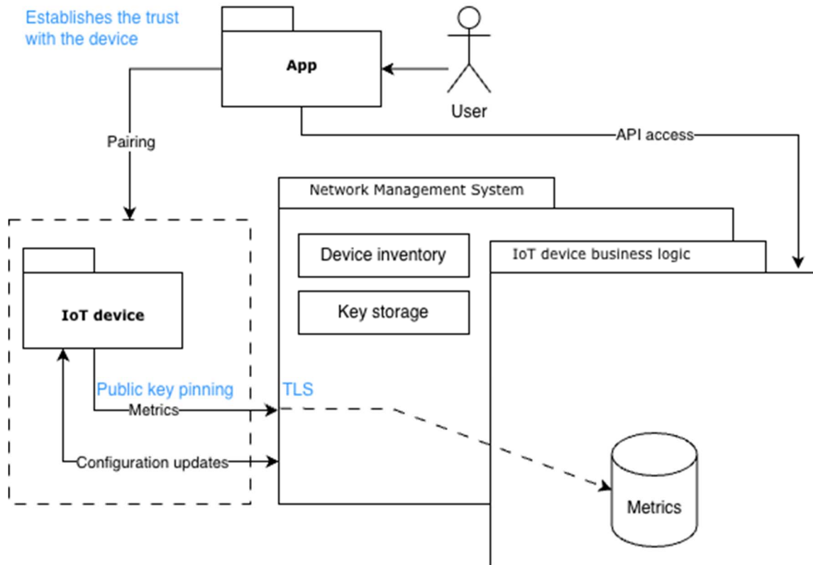
Figure 4.6.6-1: IoT network with monitoring data collection
