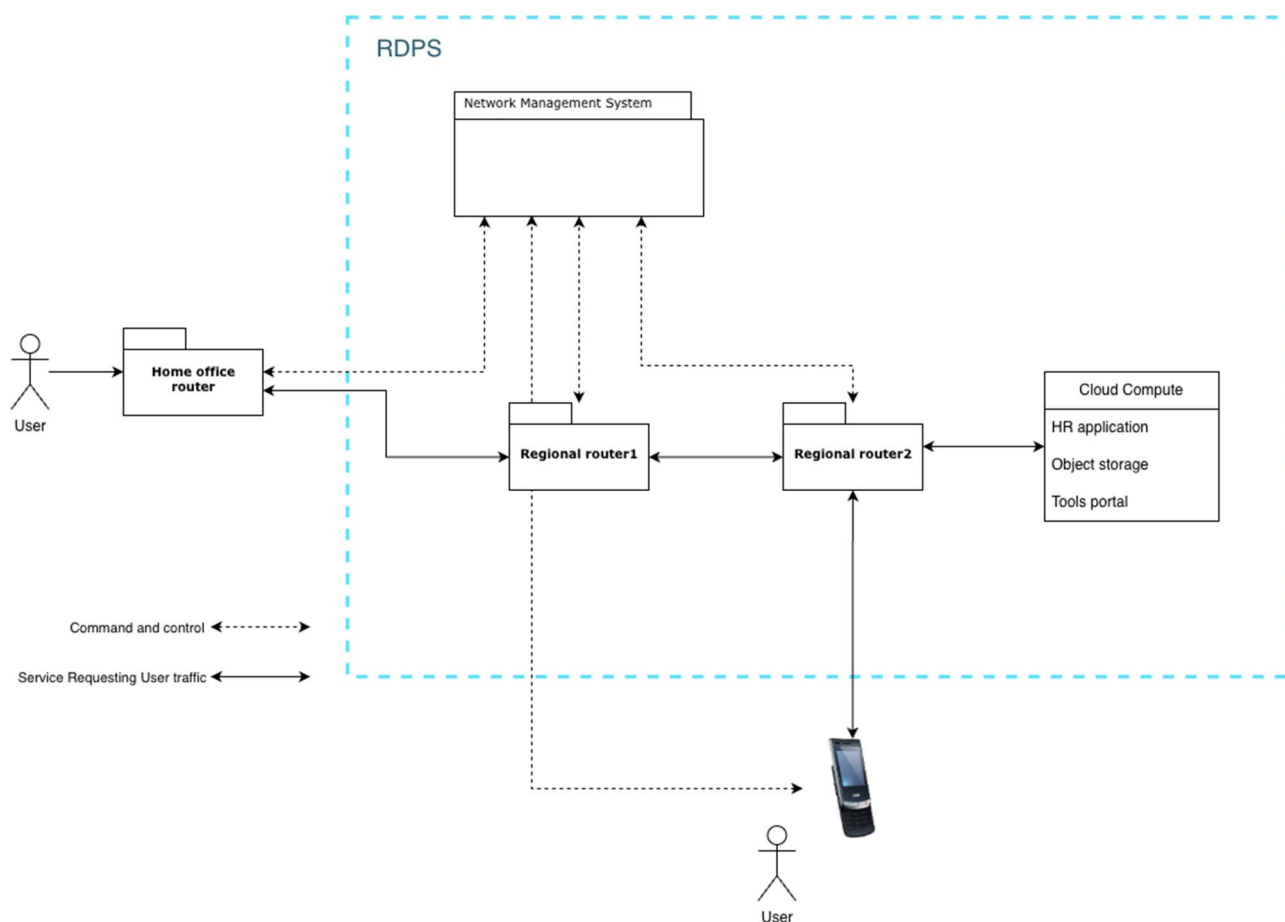
Figure 4.6.5-1: Maximum RDPS involvement
