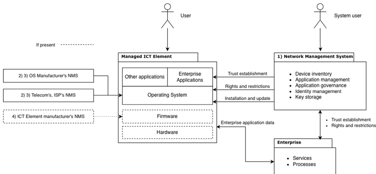
Figure 4.6.7-1: Multiple Network Management Systems
