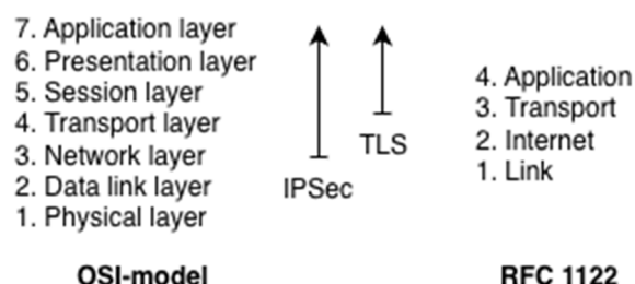
Figure 4.2.3-1: OSI-model and IETF RFC 1122
