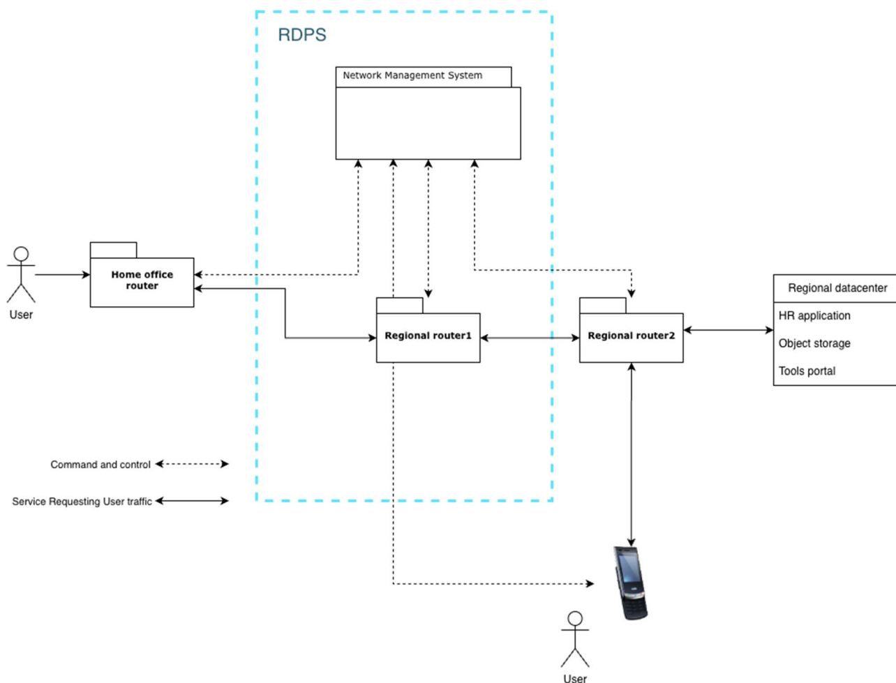
Figure 4.6.5-2: Medium RDPS involvement
