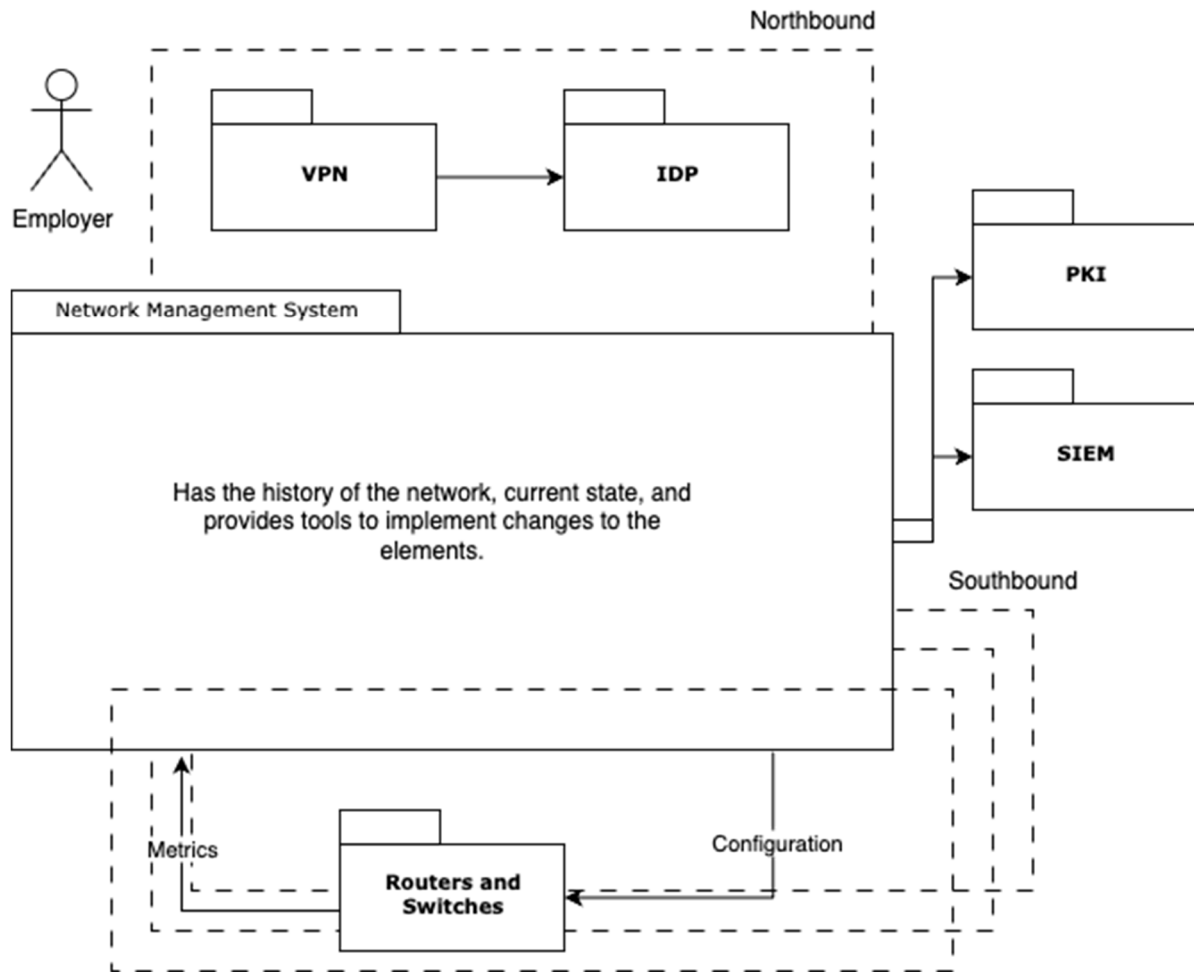
Figure 4.6.3-1: Telecommunications network
