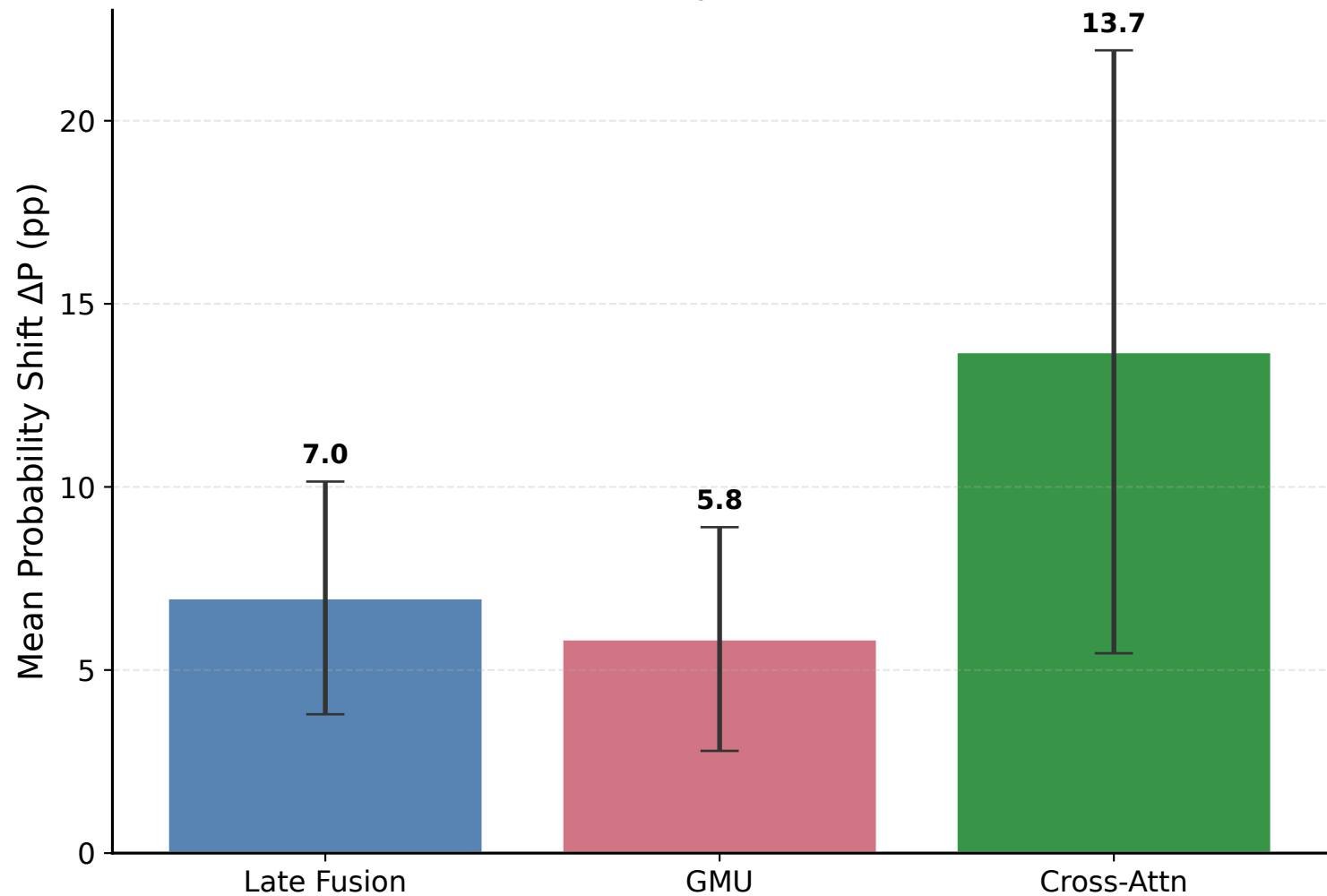
Mean \Delta P Under Counterfactual Override (95% CI, 3 Seeds)
