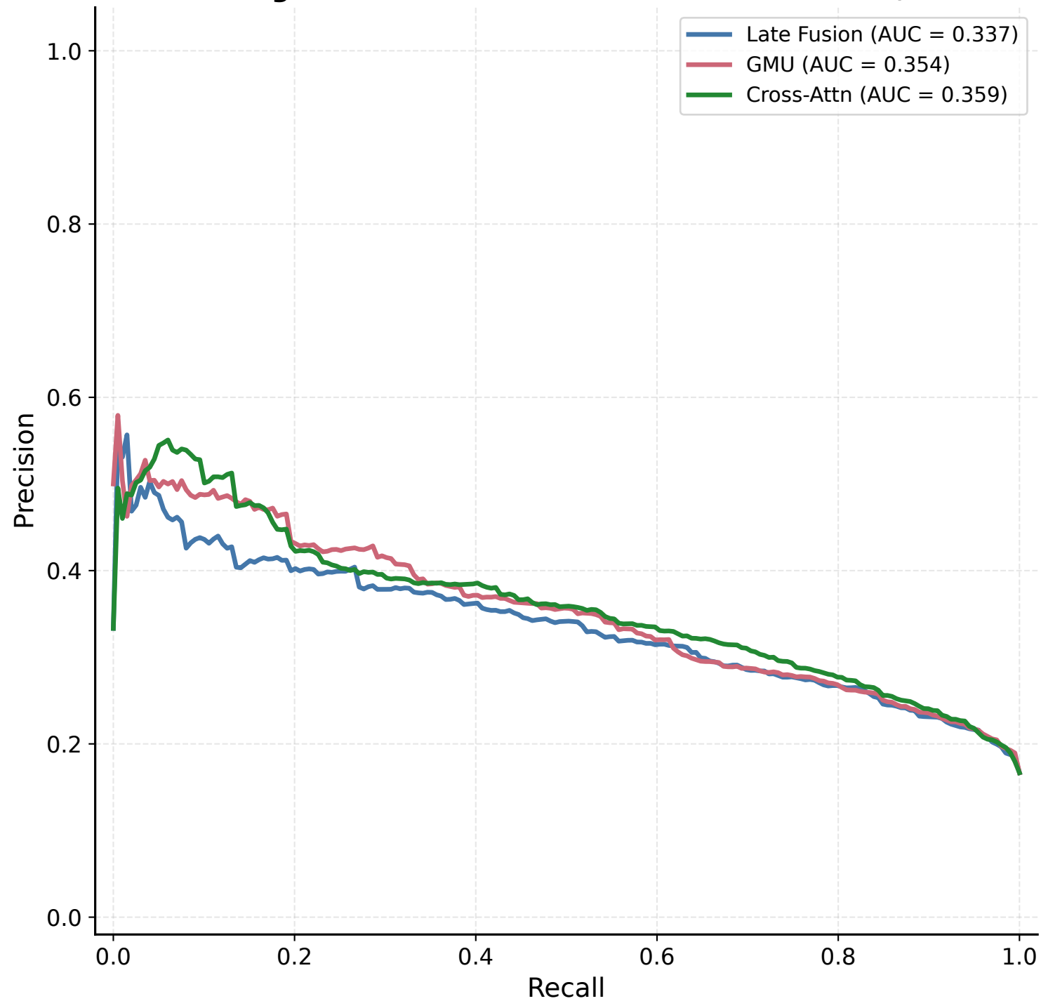
Macro-Averaged Precision-Recall Curves (PAD-UFES-20, Seed 42)
