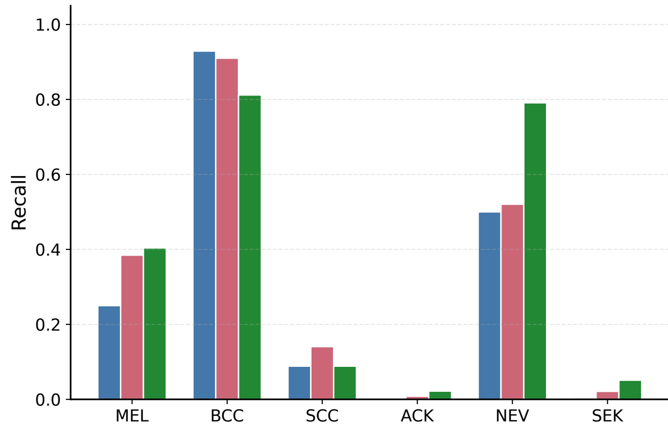
Class Accuracy
