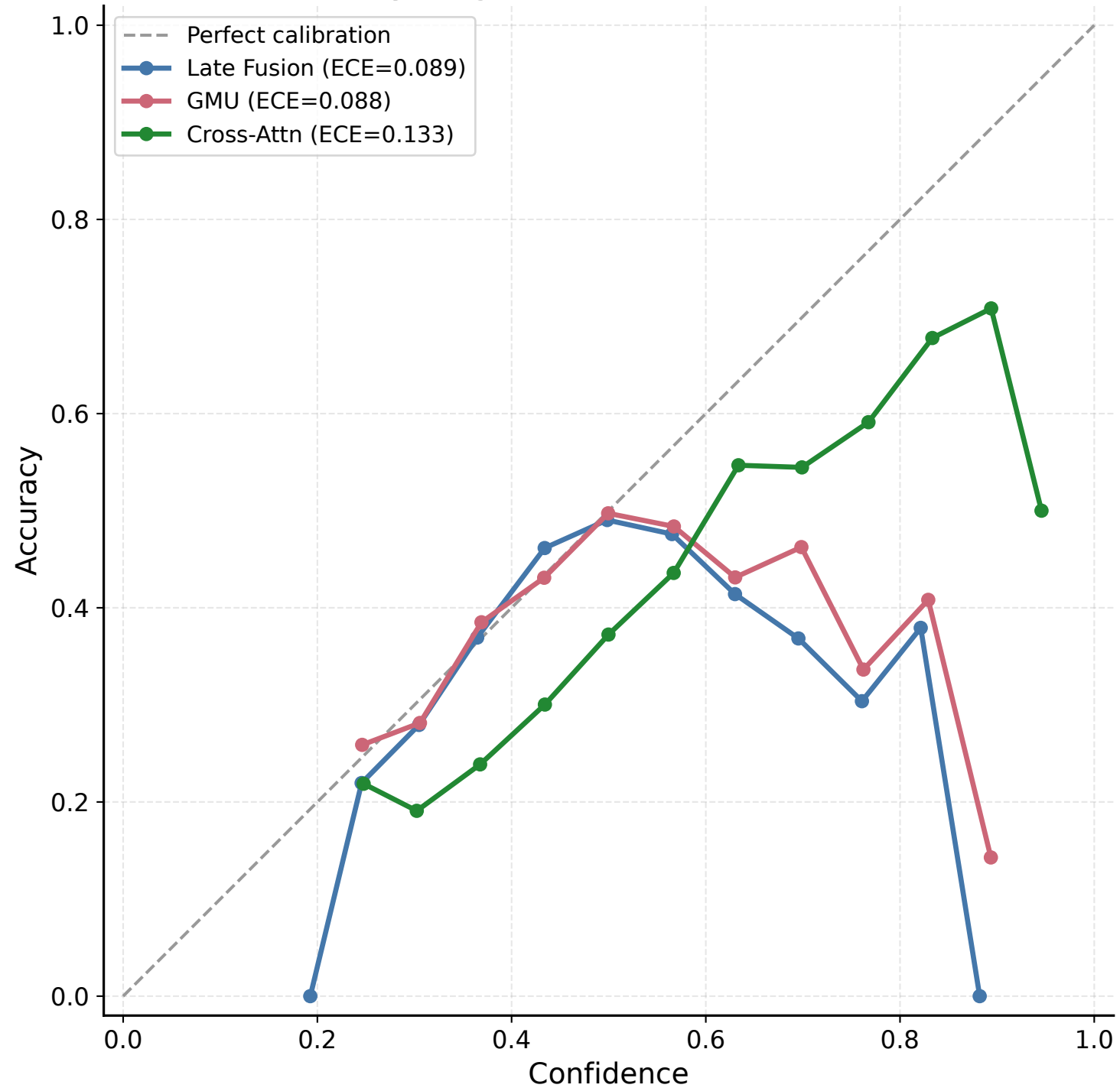
Reliability Diagrams (PAD-UFES-20, Seed 42)
