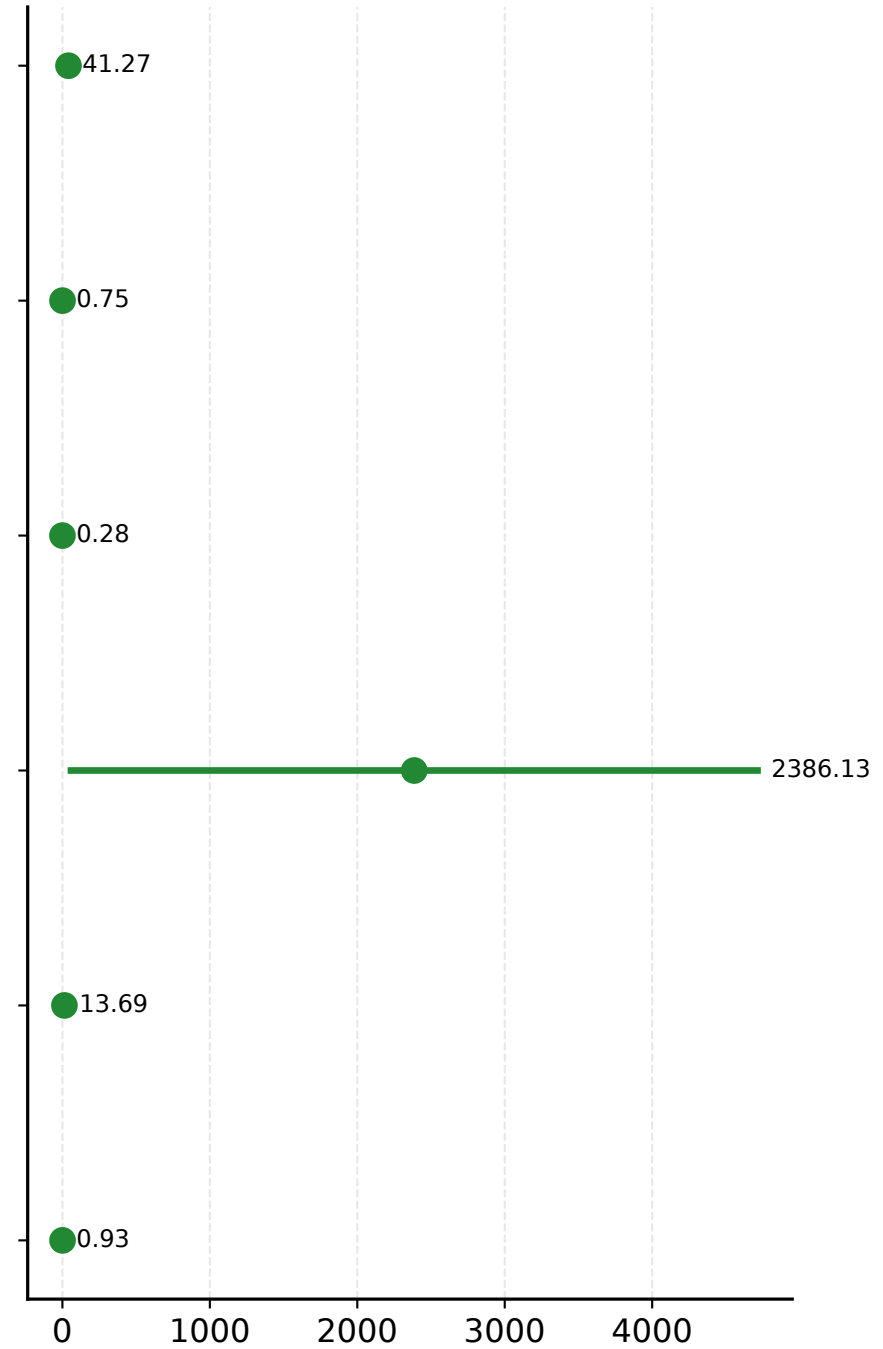
Cross-Attn
