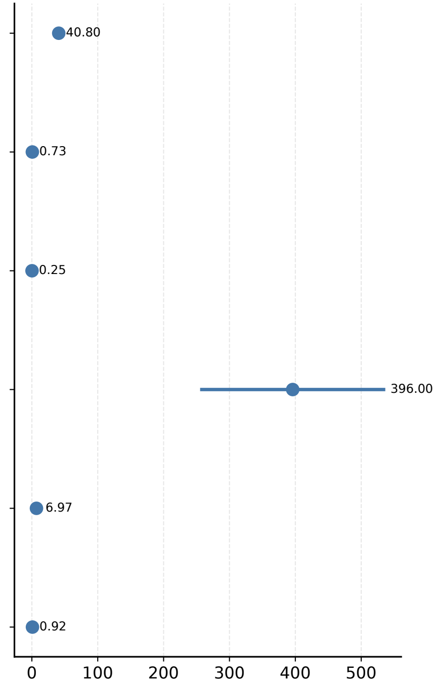
Late Fusion
