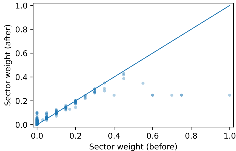
gemini-2.5-flash Pearson r=0.86
