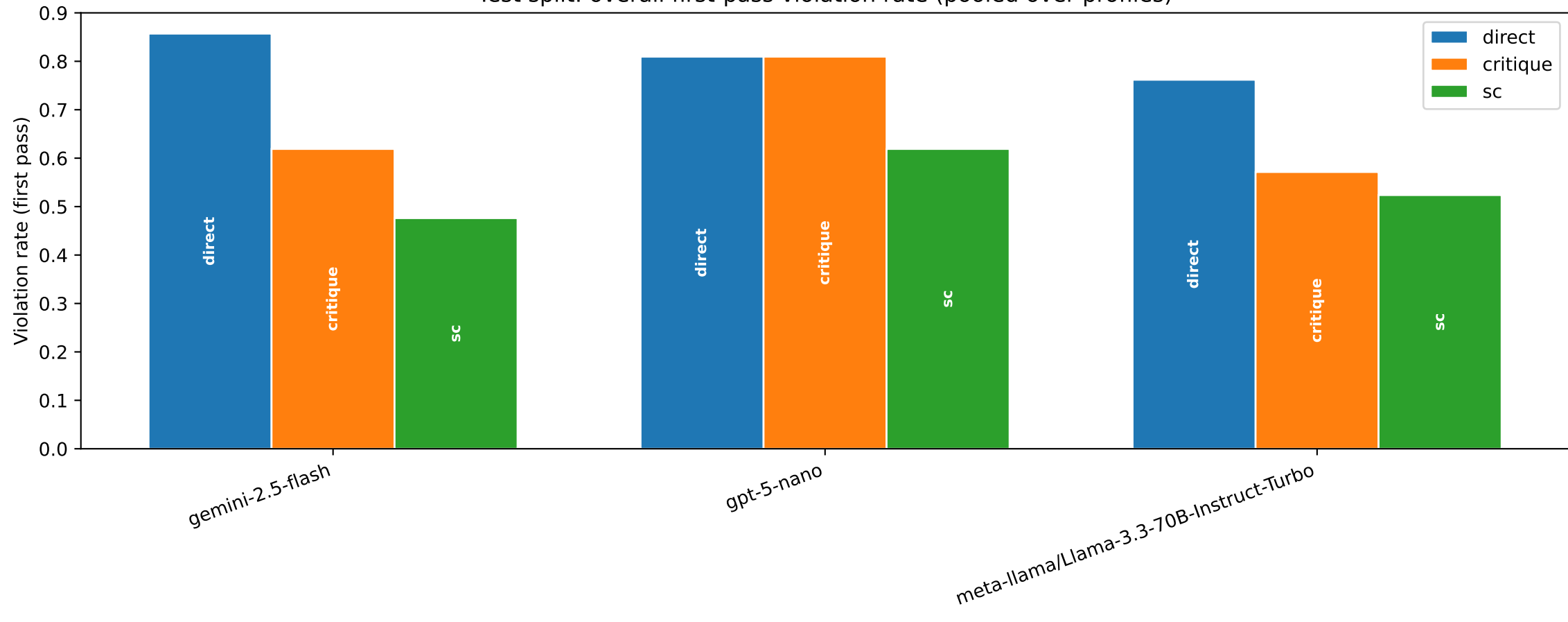
Test split: overall first-pass violation rate (pooled over profiles)
