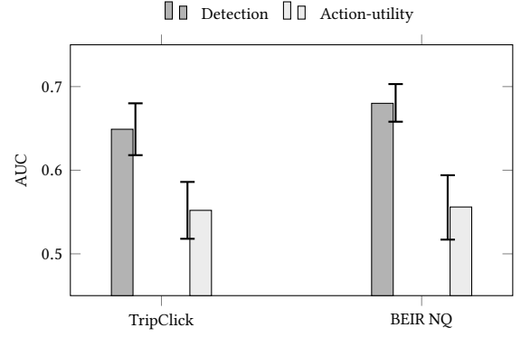
Figure 1: Table 1 as bars with 95% CIs. Detection’s CI is entirely above Action-utility’s on both corpora — the asymmetry, not just the point estimates, replicates.
