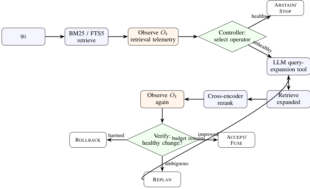
Fig. 1. The observability-guided control loop. Telemetry O_t (orange) is computed after every retrieval, not only at the end of an episode, and is causal input to two decisions: which operator the controller selects, and whether the resulting ranking is accepted, rolled back, replanned with a different operator, or the episode is stopped. The static comparator (Section VI) executes the same component chain once, with no path back from VERIFY to the LLM tool.
