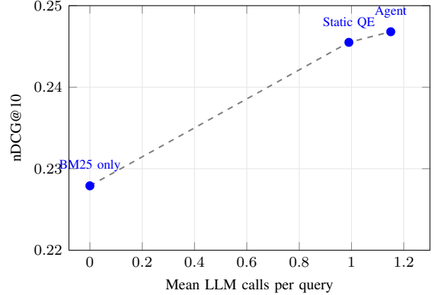
Fig. 3. Retrieval quality vs. LLM-call budget, full TripClick TAIL test set. Static QE captures nearly all of the achievable quality gain over BM25 for a fixed one-call budget; the agent’s additional 16% call overhead buys a nDCG@10 improvement (+0.0013) that is not statistically distinguishable from zero (Section VI).
