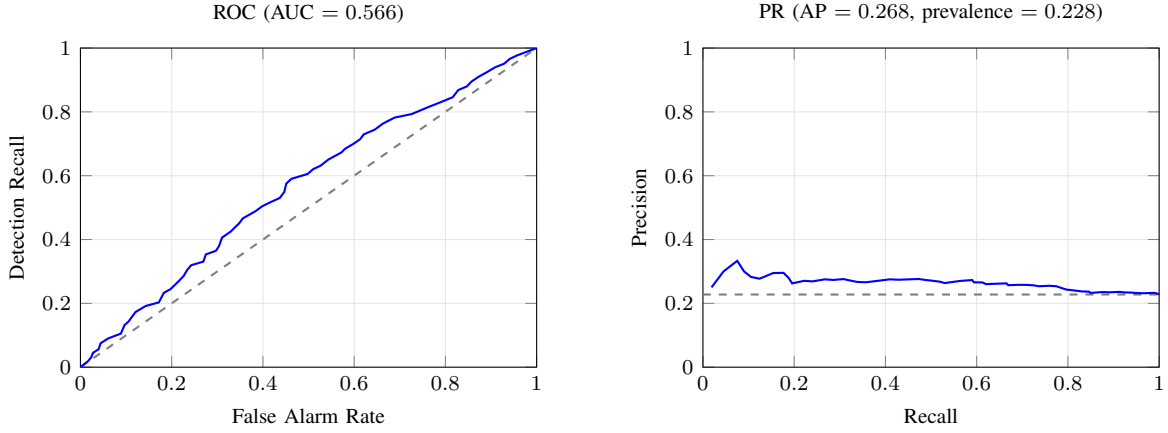
Fig. 2. Detection ROC and precision-recall curves for the deployed verifier’s score against ground-truth harm (true nDCG@10 \Delta < 0 ), swept across all thresholds on the n = 1168 calibration set. The curve sits consistently, but only modestly, above the no-skill baseline in both panels (dashed) — a visual complement to Table I’s Pearson correlations, showing the same weak-but-real signal as an operating-point trade-off rather than a single summary statistic.
