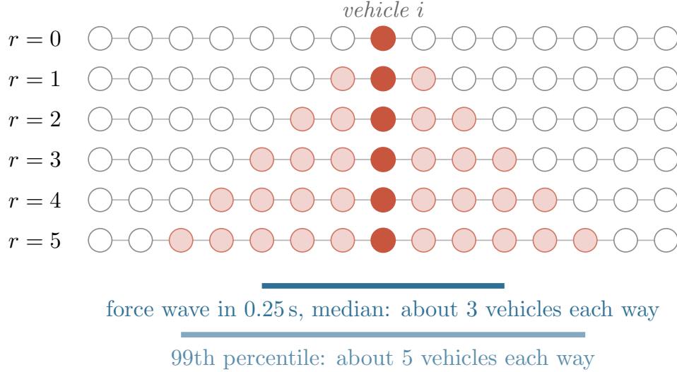
Figure 8.5: Receptive field of vehicle i after r rounds of message passing. After r rounds it has received information from vehicles up to r couplers away, and no further. A coupler force wave travels 167–193 m/s, about three vehicles each way in one 0.25 s step at the median and five at the 99th percentile over a 17 m car pitch, so five rounds cover the physical reach of one step.
