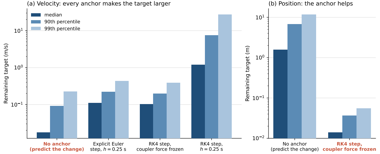
Figure 8.1: The size of the remaining learning target under each anchor, on a logarithmic scale. (a) For velocity, every physics anchor leaves a larger target than predicting the change directly. (b) For position, anchoring on the physics reduces the target more than a hundred-fold. The best choice in each panel is marked in red. Data from tables 8.1 and 8.3.
