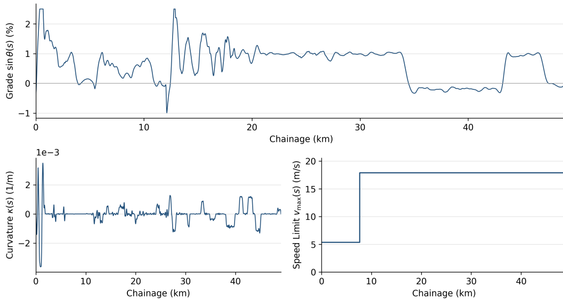
Figure 5.7: The three derived fields the simulator consumes for route_line0 , plotted against chainage in kilometres: grade \sin \theta(s) as a percentage (top), the curvature proxy \kappa(s) (bottom left), and the speed limit v_{\max}(s) (bottom right). Fields are shown after the corridor check of section 5.4, with an 800 m smoothing window and a 2.5% grade limit. The noisier grade over the first 20 km is the urban approach, where frequent bridges, junctions, and short mapped segments degrade the elevation signal; beyond it the line settles onto a sustained climb near one percent. The grade reaches the 2.5% limit only in two short runs, near the start and near 12.7 km, which are residual artifacts rather than terrain. The speed limit is a step field, here rising where the line leaves restricted urban trackage.
