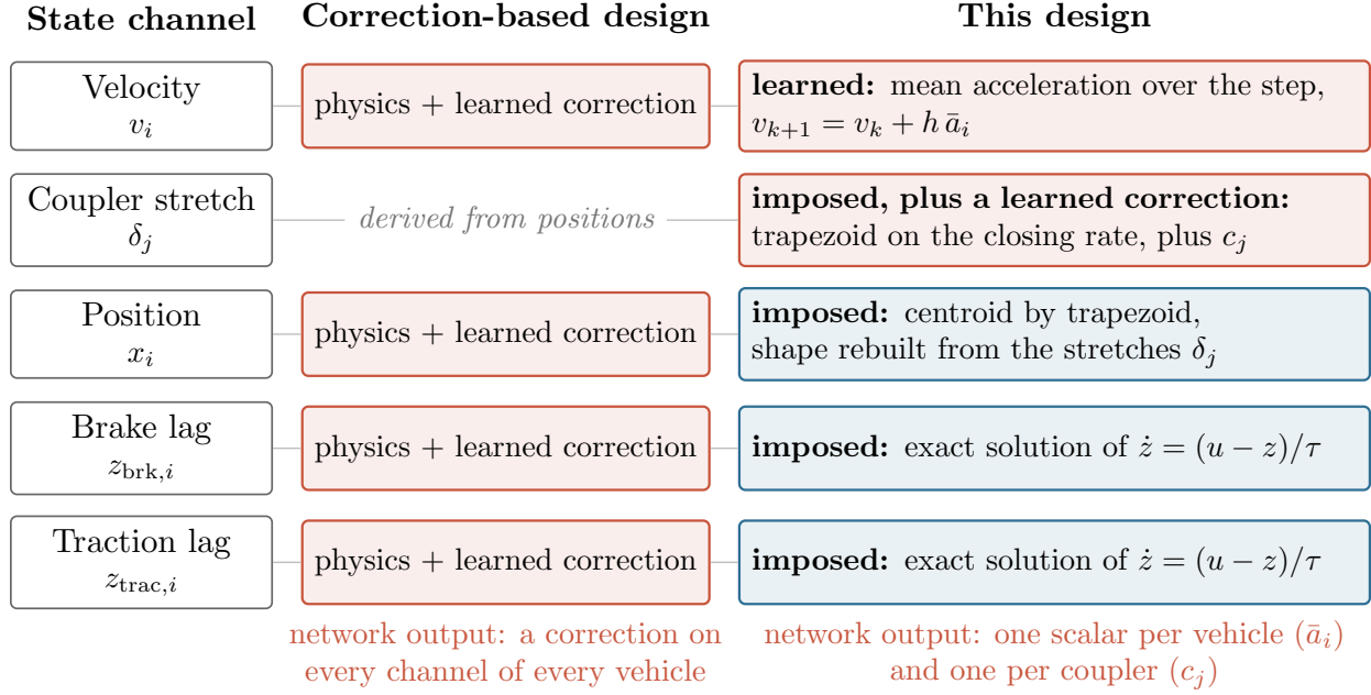
Figure 8.2: How each state channel is advanced over one step. A design that corrects the physics would learn a correction on every channel (centre). Here two channels are imposed exactly, position is imposed apart from the coupler shape, and the network’s output narrows to one scalar per vehicle and one per coupler (right).
