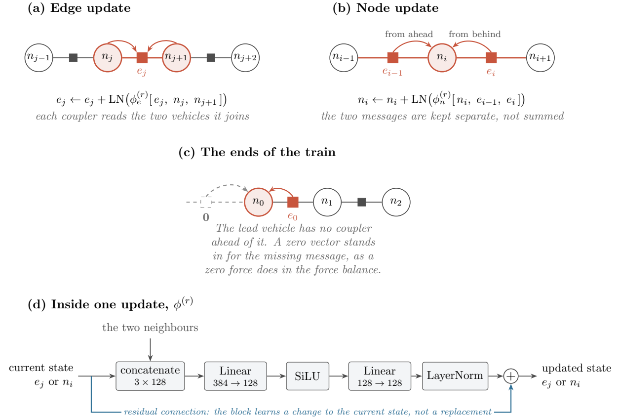
Figure 8.4: One round of message passing. (a) Each coupler updates from the two vehicles it joins. (b) Each vehicle then updates from the couplers ahead of and behind it, kept as separate inputs. (c) At the ends of the train a zero vector stands in for the missing coupler. (d) Each update is a two-layer MLP followed by layer normalization, added to the current vector through a residual connection.
