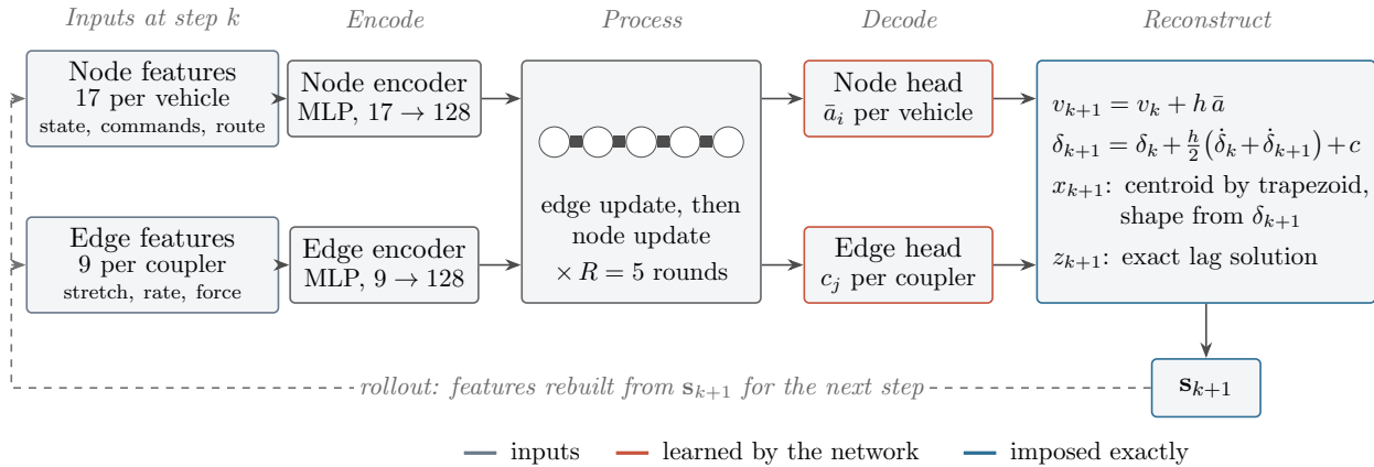
Figure 8.3: The surrogate as a whole. Node and edge features are encoded into 128-dimensional vectors, updated by five rounds of message passing along the chain, and decoded into the two learned outputs. The reconstruction step turns those into the next state exactly as in eq. (8.6). In a rollout the new state is fed back as the next input.
