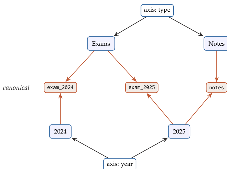
Figure 5: Two axes over the same three sources, grouping them differently: by type the sources split {exam_2024, exam_2025} against {notes}, and by year they split {exam_2024} against {exam_2025, notes}. Every accent edge is one placement block. No canonical block is copied and none of them changes, so adding, removing, or restructuring an axis touches only the semantic module and the canonical root a consumer already holds stays exactly as it was.
