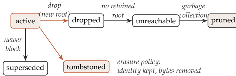
Figure 10: Lifecycle states of a knowledge block. The ordinary removal path for non-episodic modules is drop: a new Merkle root excludes the block, provenance is updated, and pruning later reclaims bytes once no retained root references it. Supersession keeps the block in the composition; redaction destroys bytes that a retained root still names.
