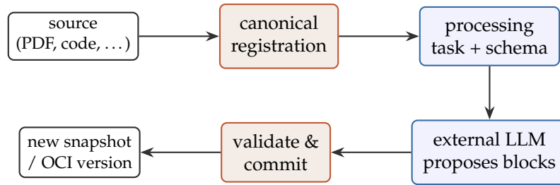
Figure 8: The brain conserves and validates; the external LLM interprets and proposes blocks. Only validated candidates are committed and versioned.
