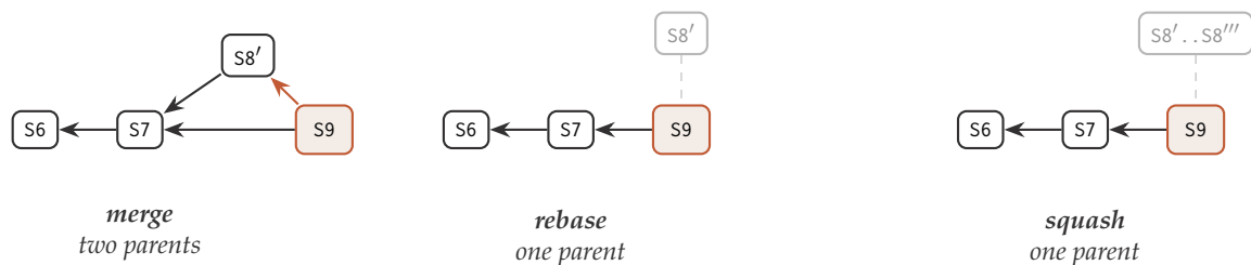
Figure 11: All three land the same blocks in S9. Only merge keeps the contributed snapshot in the history, and therefore only merge keeps the contributor's signature covering something. Greyed nodes are outside the resulting history.
