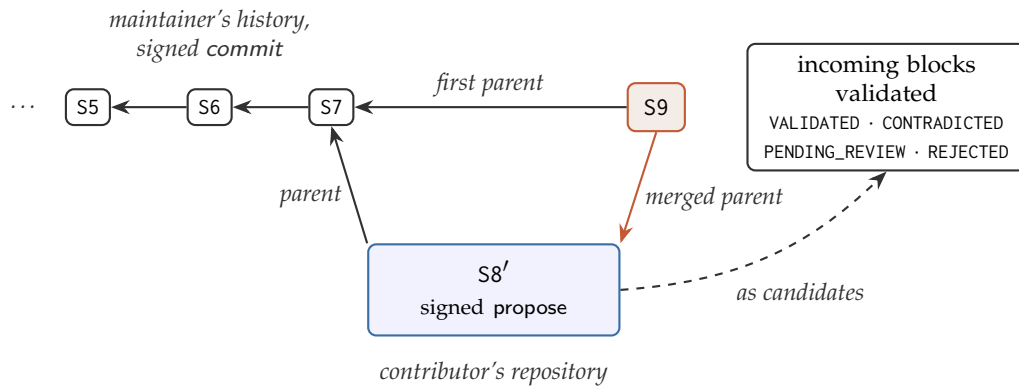
Figure 12: An external contribution needs no new object. The contributor's snapshot names a snapshot of the maintainer's history as its parent, which is the whole link; the maintainer fetches only the delta, validates the incoming blocks as candidates, and records the outcome as a reconciliation whose first parent is their own history.
