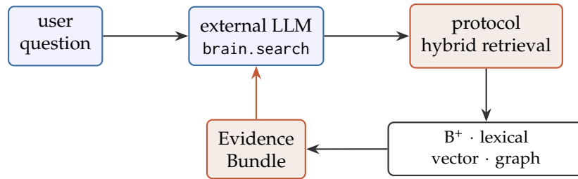
Figure 9: The external LLM queries the brain and contextualizes the returned Evidence Bundle. The protocol combines indices, verifies hashes, and returns data rather than prose.
