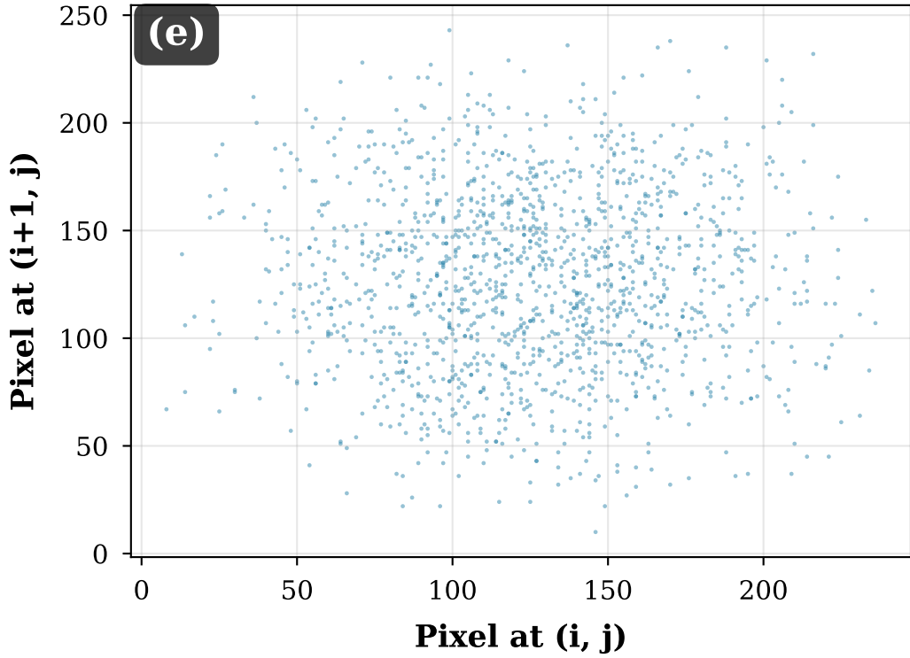
Correlation Vertical (Coef. = -0.0308)
