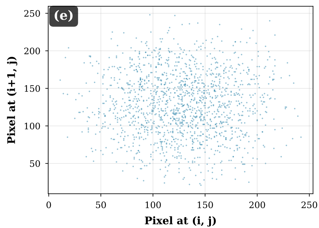
Correlation Vertical (Coef. = -0.0004)
