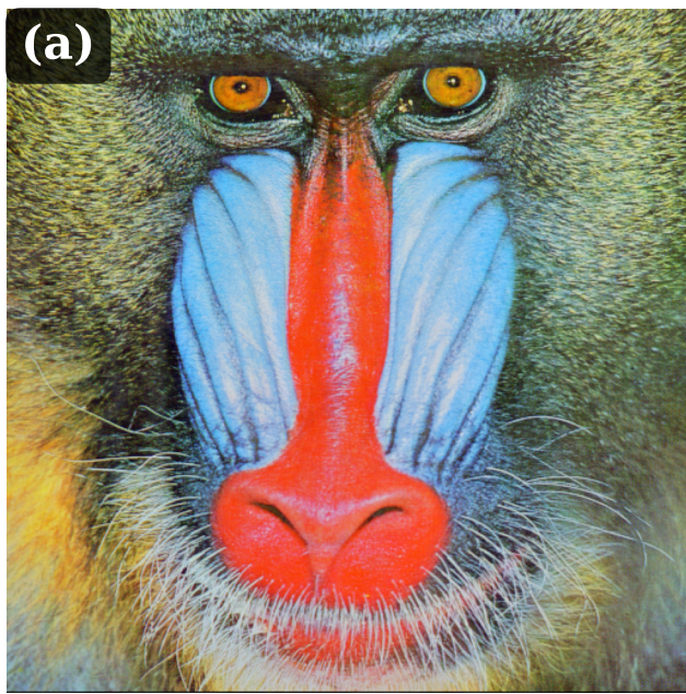
Original Image
