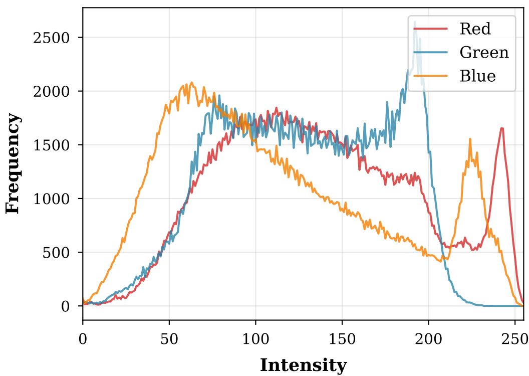
Histogram - Original
