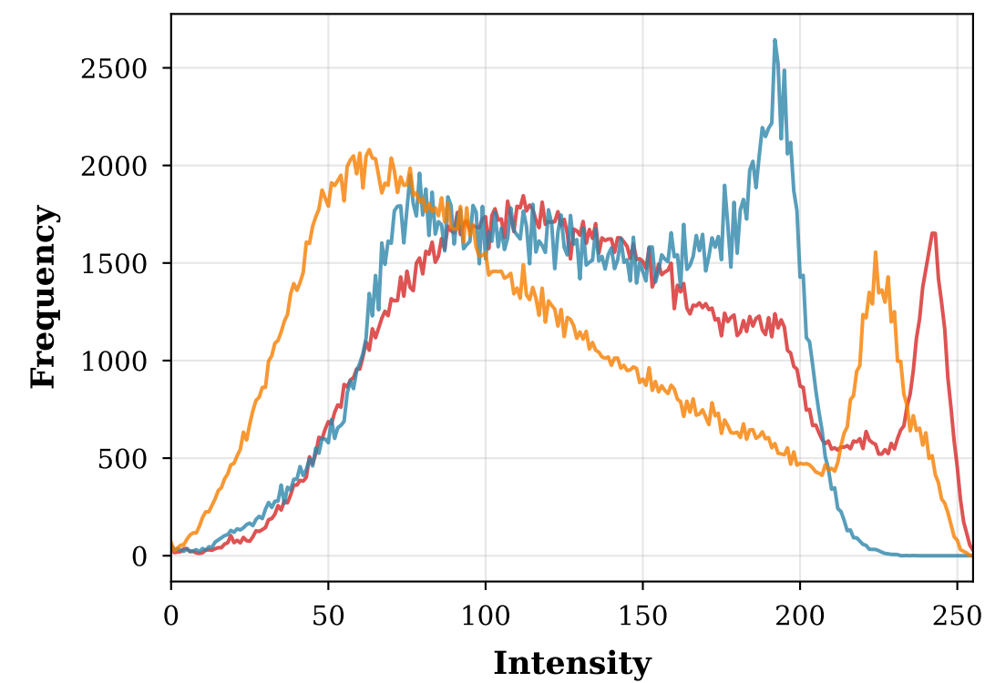
Histogram - Decrypted
