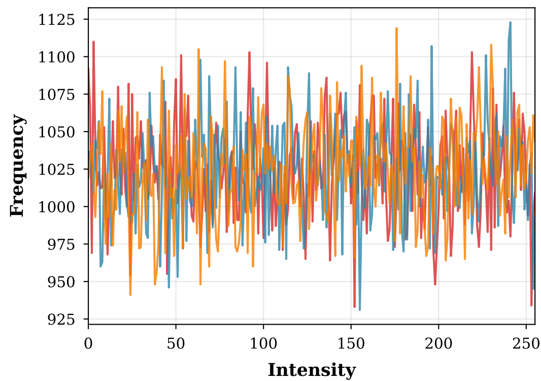
Histogram - Encrypted
