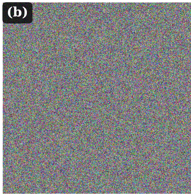
Encrypted Image
