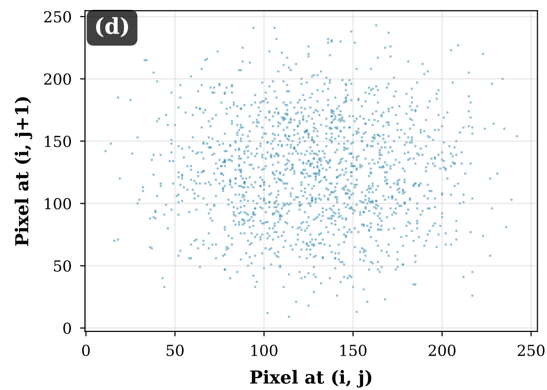
Correlation Horizontal (Coef. = -0.0174)
