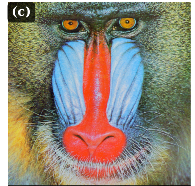
Decrypted Image
