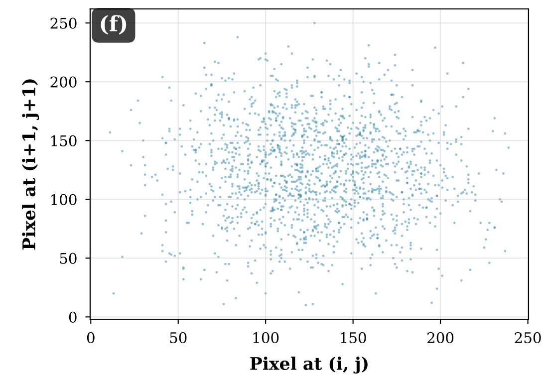
Correlation Diagonal (Coef. = 0.0062)
