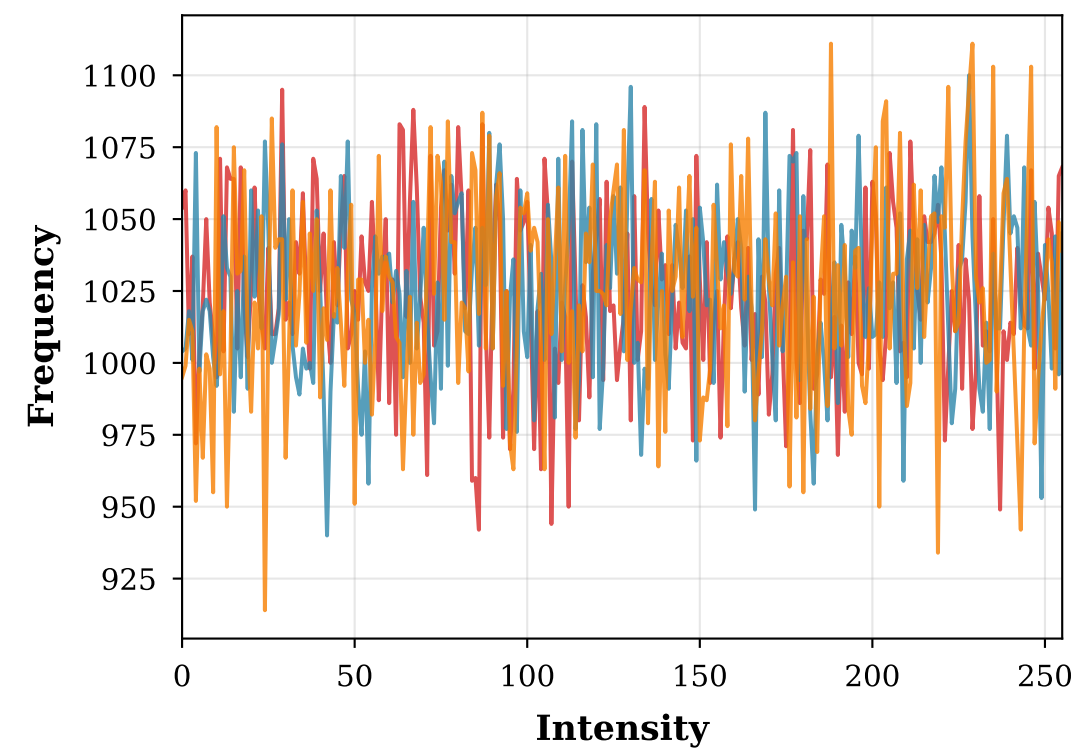
Histogram - Encrypted
