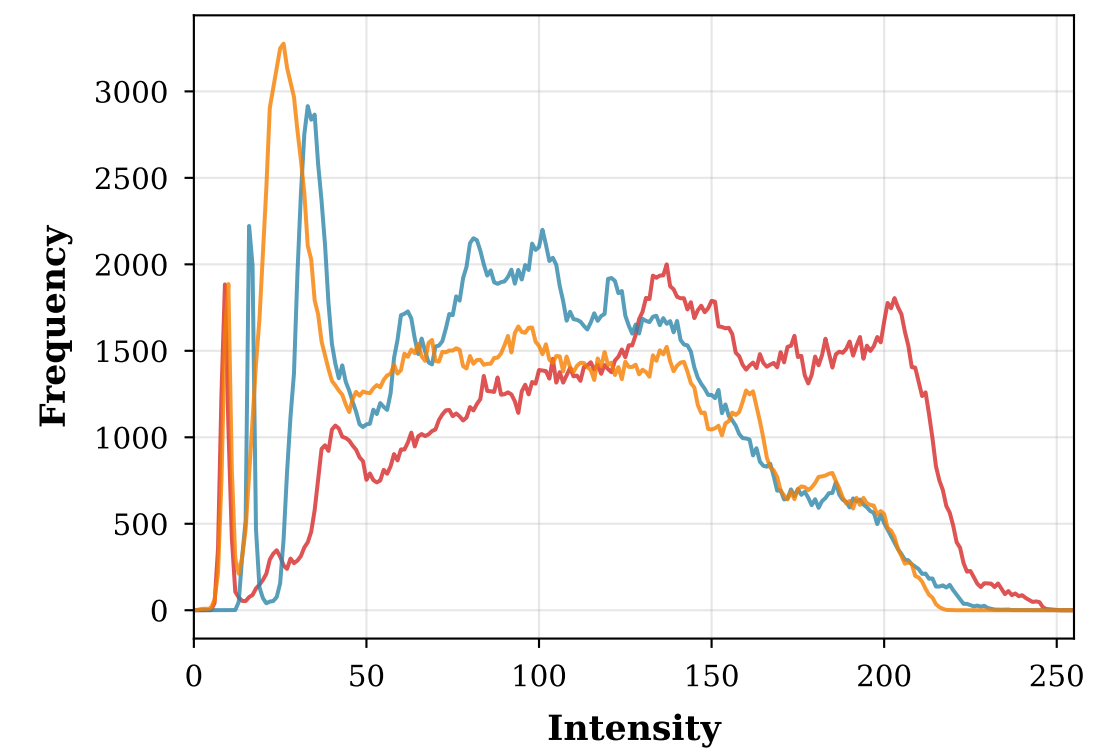
Histogram - Decrypted
