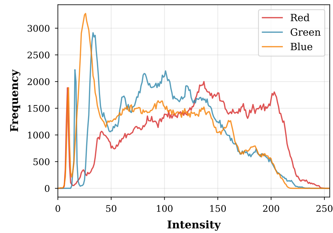
Histogram - Original
