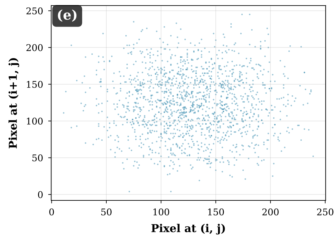
Correlation Vertical (Coef. = -0.0175)
