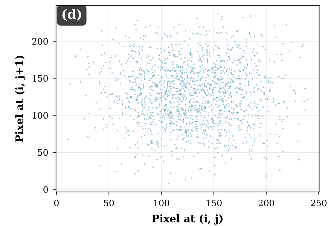
Correlation Horizontal (Coef. = 0.0654)
