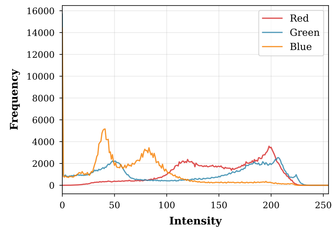
Histogram - Original
