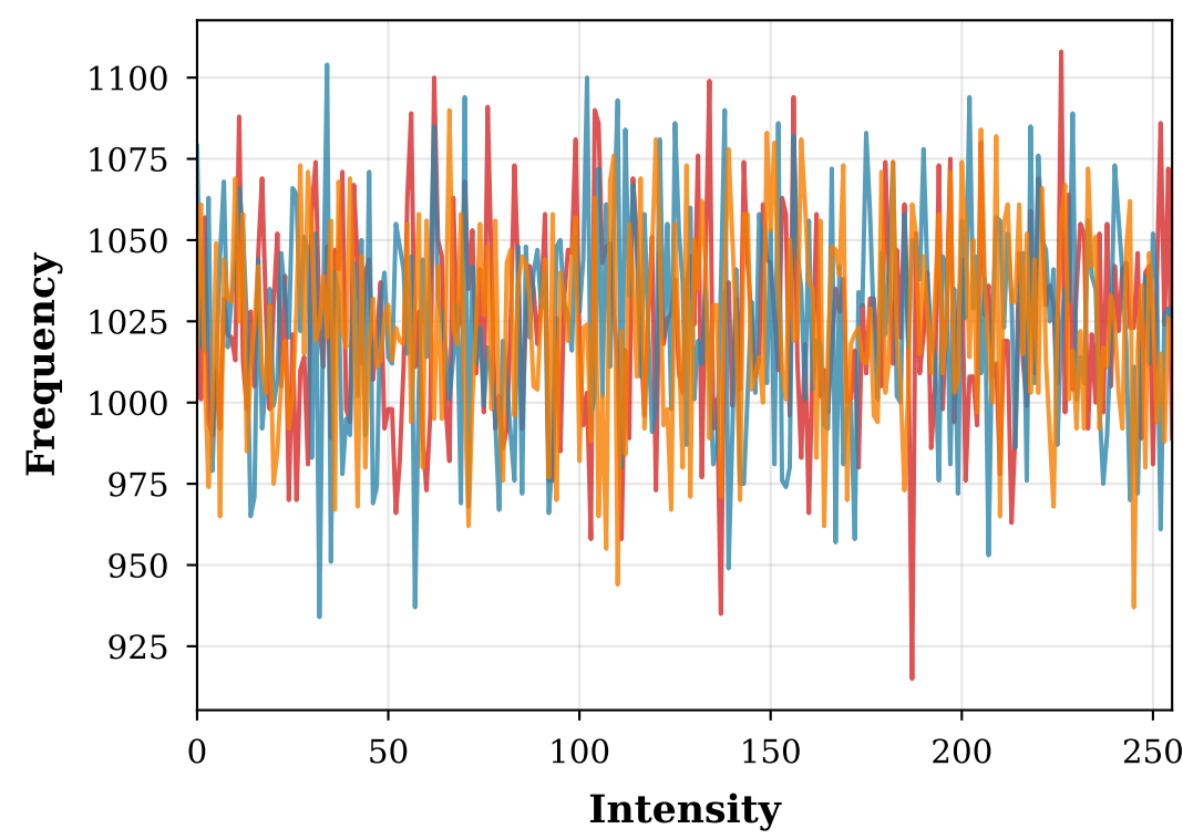
Histogram - Encrypted
