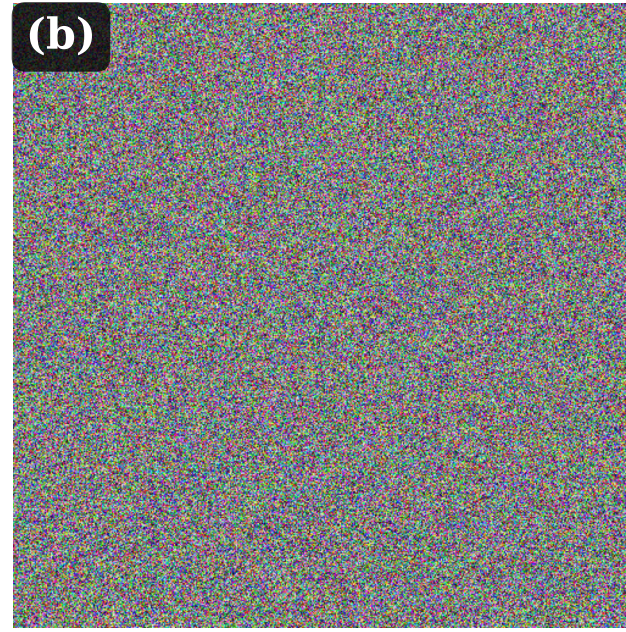
Encrypted Image
