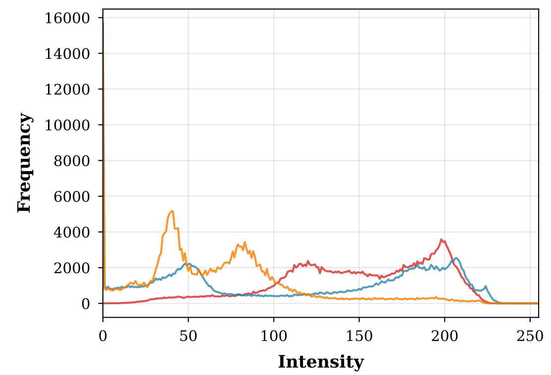
Histogram - Decrypted
