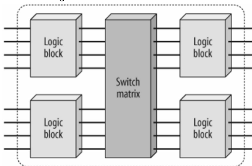
Figure 13-4. CPLD internal structure
