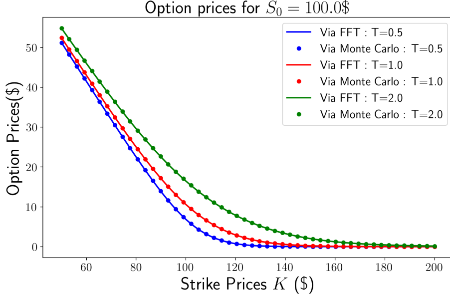
Figure 2: Here we compare the option prices obtained via the FFT to the Option prices obtained via the Monte Carlo simulations. The spot price was fixed at S_0 = 100\$ and calculations were performed for T = 0.5, 1.0, 2.0 respectively. The parameters used for these simulations were r = 0.05, \sigma = 0.15, \lambda = 1.5, \eta_1 = 25.0, \eta_2 = 10.0 .
