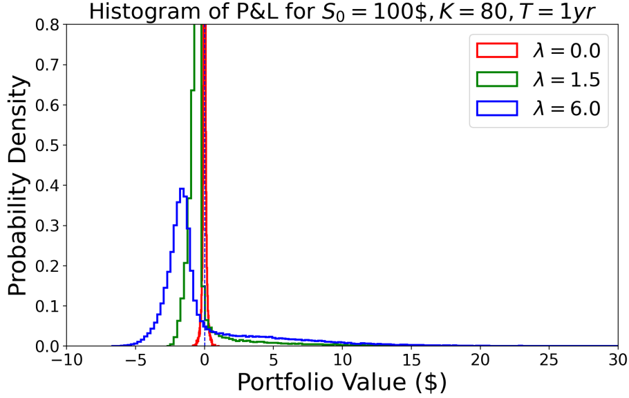
Figure 3: Here we compare the values of delta-hedged portfolios. The spot price was fixed at S_0 = 100\$ , strike price at K = 80\$ and time to expiry was T = 1 (year). The parameters used for these simulations were r = 0.05, \sigma = 0.15, \eta_1 = 25.0, \eta_2 = 10.0 , while \lambda was selected as 0.0, 1.5, 6.0 respectively. The hedged position was adjusted twice every working day. The vertical dashed line represents the mean for each \lambda , which is 0 $ for all three cases as expected.
