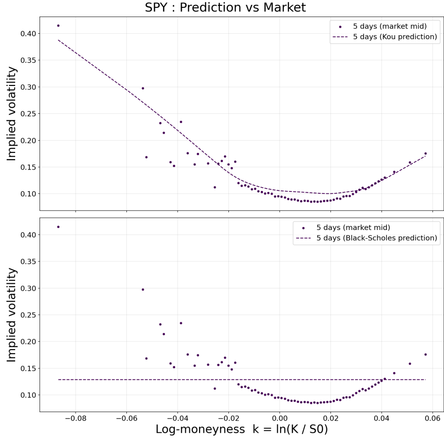
Figure 1: Implied volatility is plotted against log-moneyness. The scatter plots are the test data and the dashed lines refer to the model predictions. The upper figure shows the results for the Kou Model and lower figure shows the results for the black-scholes model
