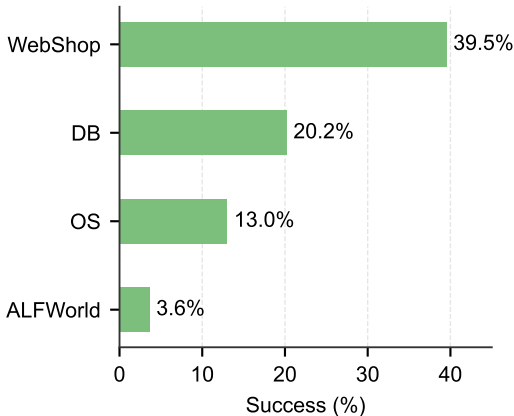
(c) Success by domain
