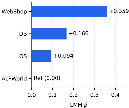
(c) Domain effect ( \hat{\beta} )
