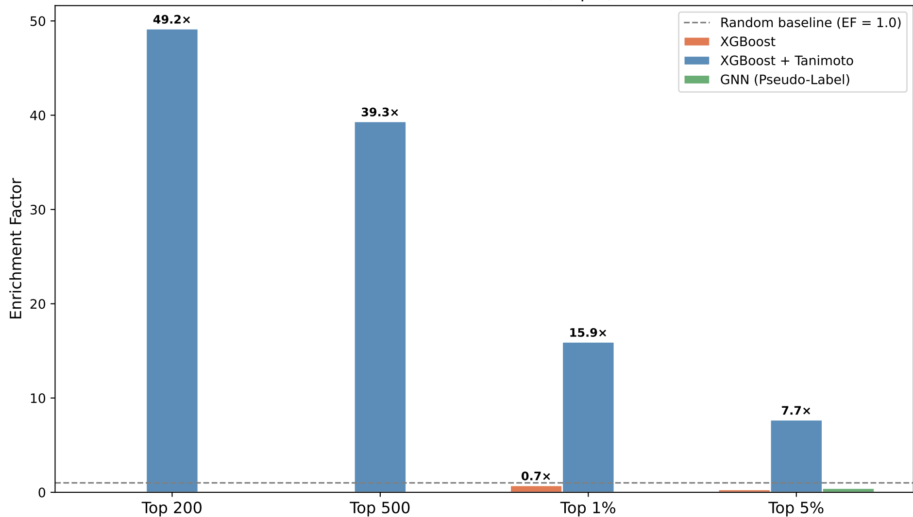
EF on 138 Confirmed WDR91 Actives (Step 2) — All Methods
