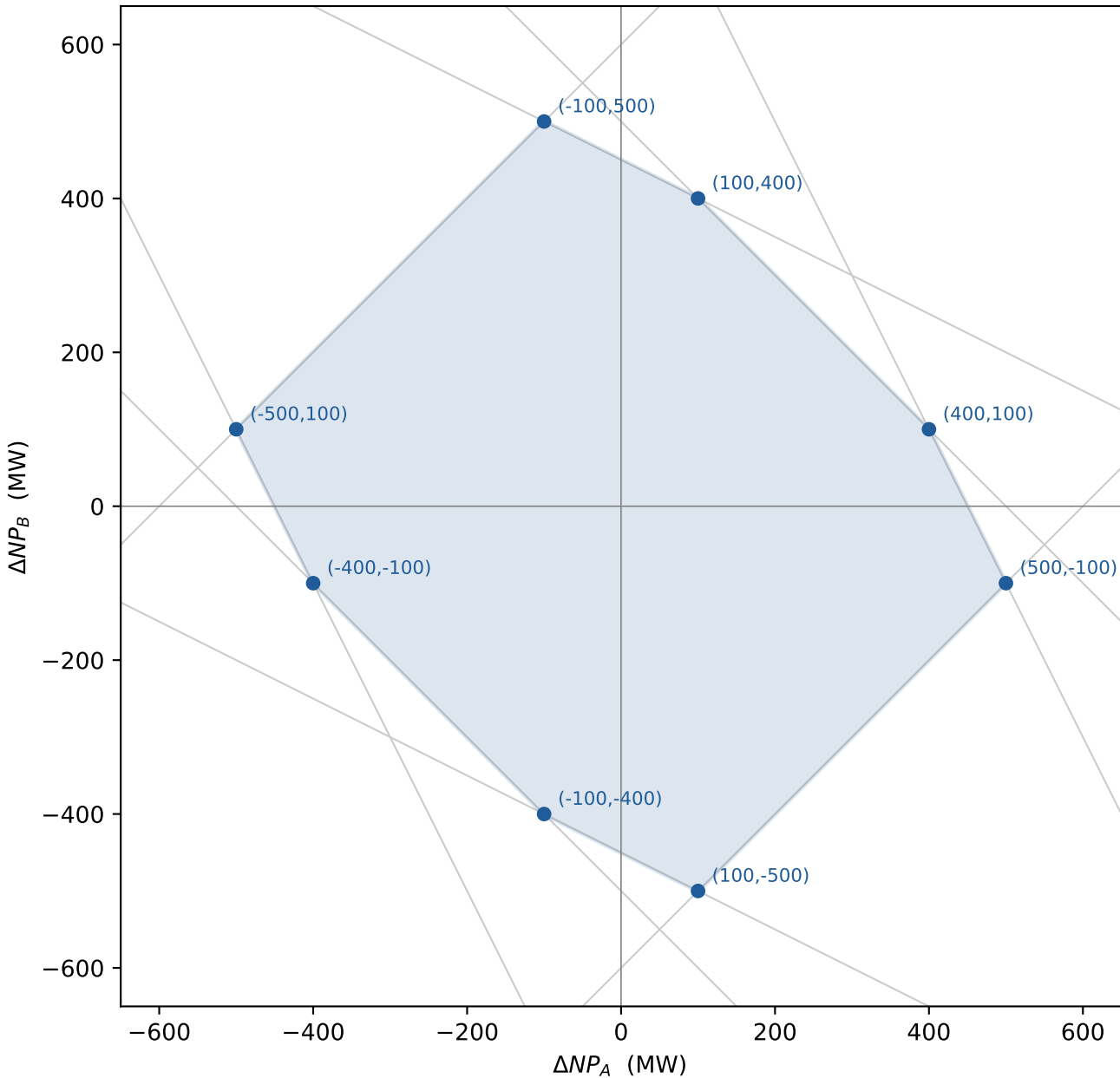
Domaine flow-based (PTDF & RAM issus de pypowsybl)
