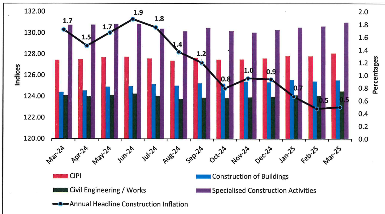
Figure 1: Annual Headline Construction Sector Inflation: March 2024 – March 2025
