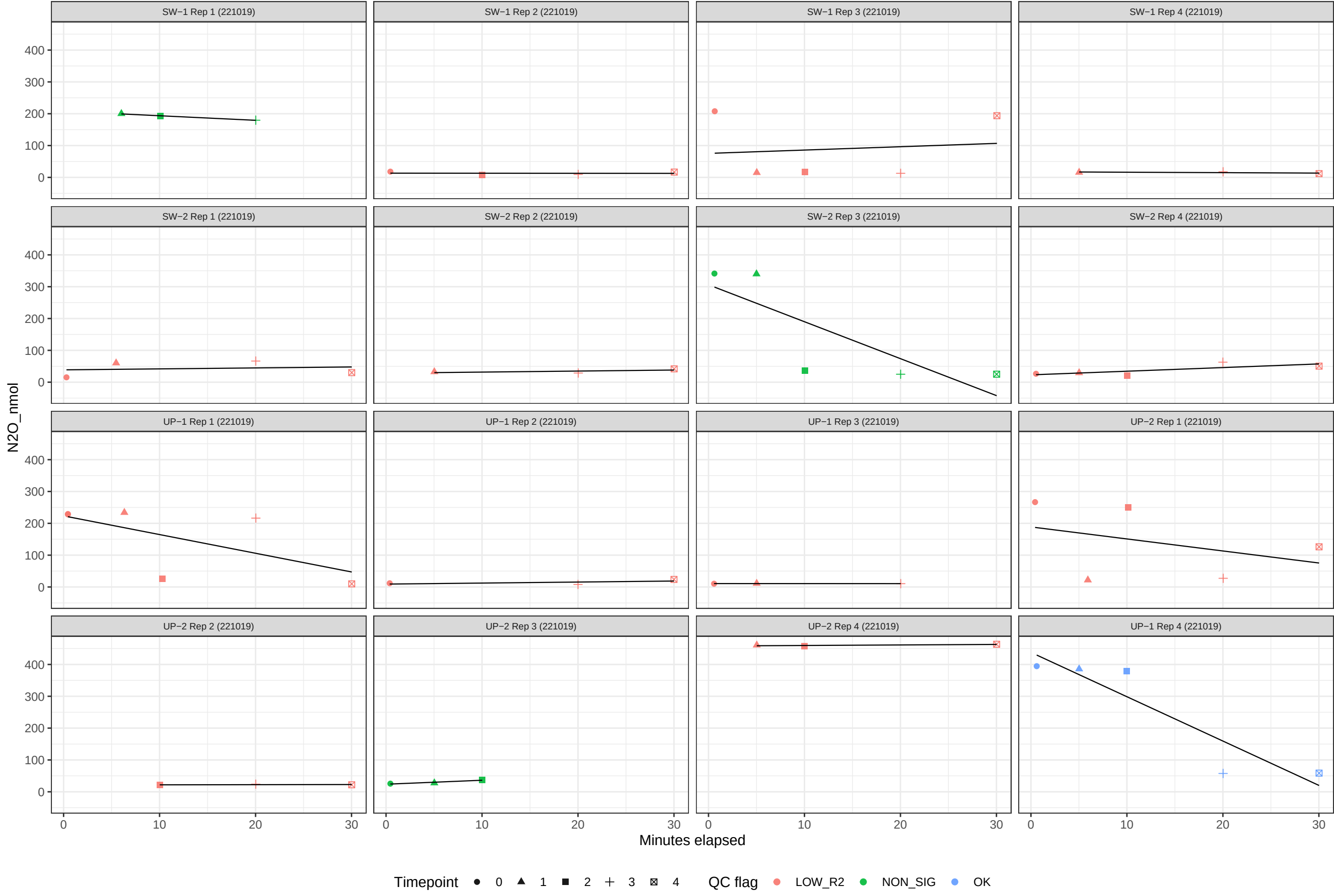
All chamber series (QC-colored): N2O_nmol | 221019 Black line = LM fit per chamber-series; points colored by qc_flag (OK vs non-OK).
