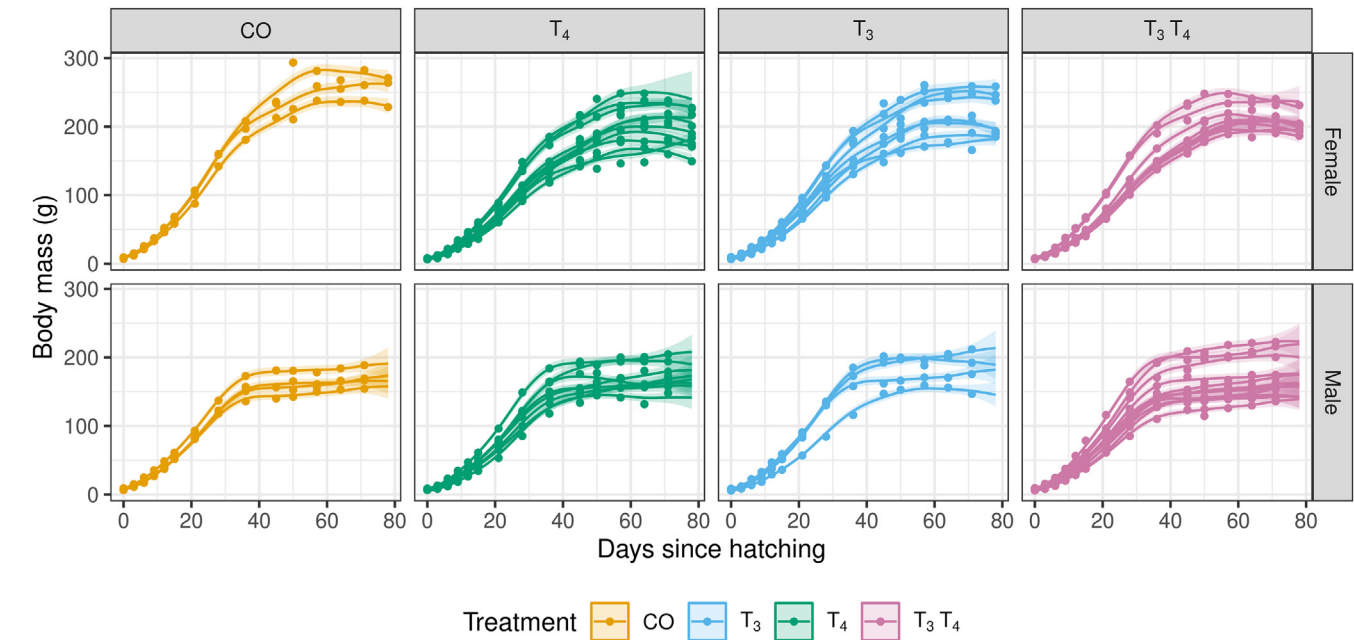
Fig. 7. Measured body mass (g) for 57 Japanese quail from an experiment on the effects of exposure to the maternal hormone T_4 , its active metabolite T_3 , both ( T_3 T_4 ) or a saline solution control (CO). The data (points) are shown alongside the estimated growth curve for each quail obtained using generalized additive model Q3, which are shown by the coloured lines in each panel. The coloured shaded ribbon is the 95% Bayesian credible interval around the estimated curve. The data are faceted by treatment and the sex of bird.
