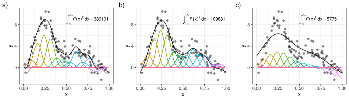
Fig. 2. Illustration of how the wiggliness penalty controls the resulting fit of a penalised spline. The weighted basis functions are shown as thin coloured lines. In each panel, a penalised spline is shown by the solid black line, which has been fitted to the data points shown. The wiggliness value of the spline, the integrated squared derivative of the fitted spline over x is given in the upper right of each panel. The spline in (a) is overfitted to the data, resulting in a very wiggly function with a large wiggliness value. The spline in (c) is over-smoothed, resulting in a simple fitted function with low wiggliness, but which does not fit the data well. The spline in (b) represents a balance between fit to the data and complexity of fitted function. The smoothing parameter for the spline, \lambda , is used as a tuning parameter in the model, which ultimately controls this balance between fit and complexity.
