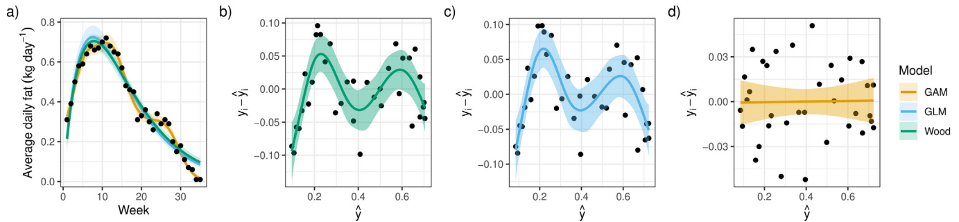
Fig. 3. Results of model fitting to the cow average daily fat content data from Henderson and McCulloch (1990). (a) observed average daily fat content (points) and estimated lactation curves from Wood's model, a Tweedie GLM, and a Tweedie GAM (lines) with associated 95% confidence intervals (Wood's model) or 95% credible intervals (GLM and GAM). Response residuals for Wood's model (b), Tweedie GLM (c), and Tweedie GAM (d), plus scatter plot smoothers (lines) and 95% credible intervals (shaded ribbons).
