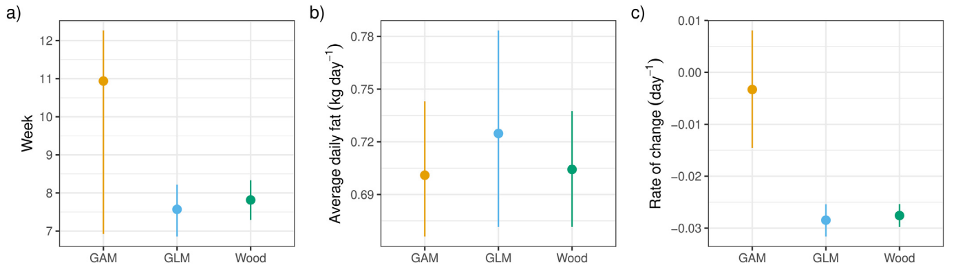
Fig. 4. Quantities of interest derived from Wood's model, a Tweedie GLM, and a Tweedie GAM fitted to the cow lactation data: (a) the estimated week of peak average daily fat content, (b) the estimated average daily fat content at the peak, and (c) the rate of change (first derivative) of the lactation curve estimated at a point that is midway between the peak fat content and the end of lactation. The points are the estimated values, and the lines are a 95% uncertainty interval. The uncertainty interval is based on the 0.025 and 0.975 percentiles of the bootstrap distribution of model coefficient estimates (Wood's model) or of the posterior distribution (GLM and GAM).
