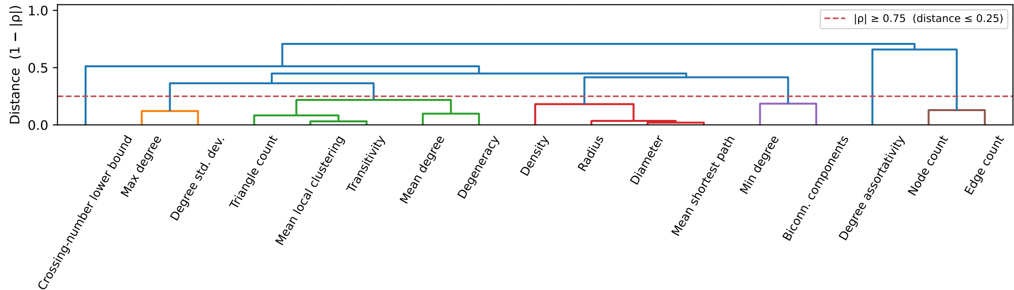
Property correlation dendrogram — Spearman \rho , average linkage
