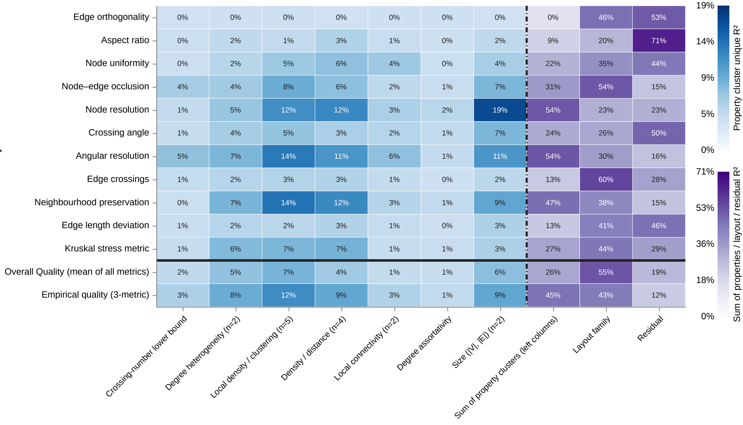
Shapley R^2 contribution of each property cluster to each readability metric
